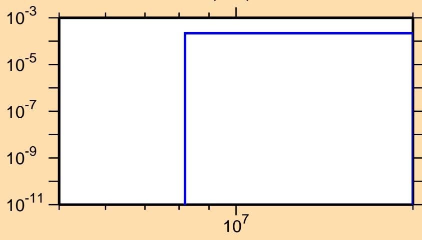
\sigma vs. E for ^{247}\text{Cf}(n,d)
