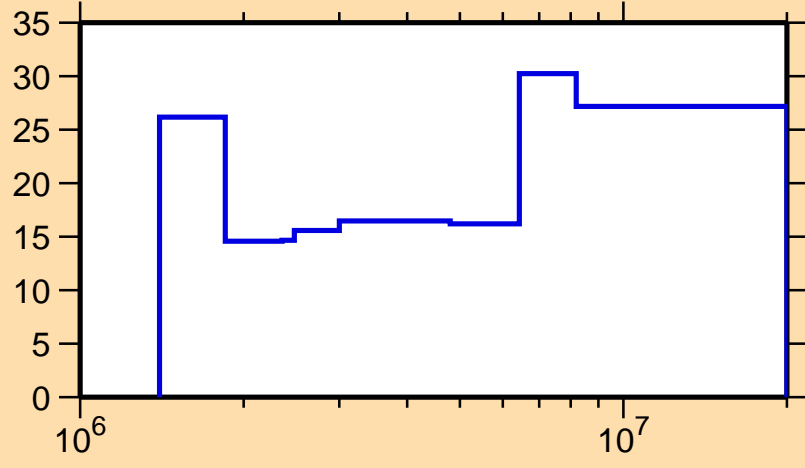
\Delta\sigma/\sigma vs. E for ^{247}\text{Cf}(n,n\text{cont.})
