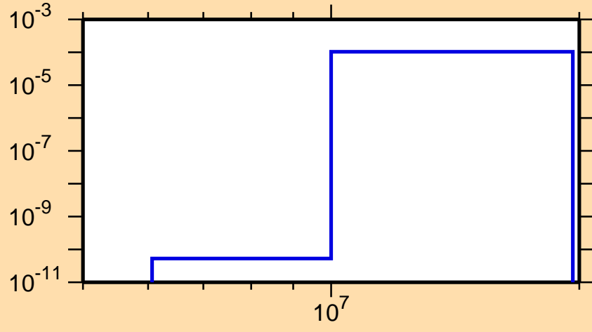
\sigma vs. E for ^{248}\text{Cf}(n,d)
