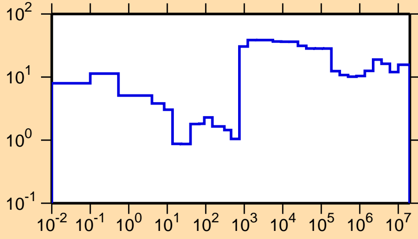
\Delta\sigma/\sigma vs. E for ^{248}\text{Cf}(n,el.)
