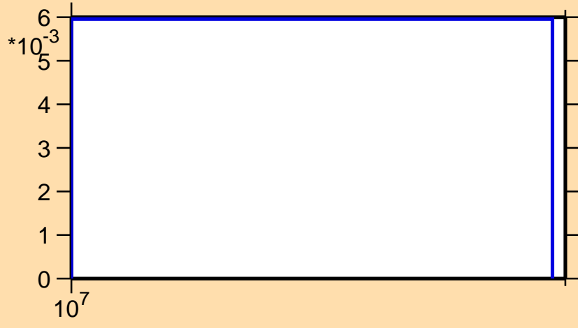
\sigma vs. E for ^{248}\text{Cf}(n,3n\alpha)
