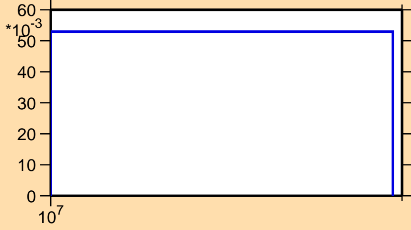
\sigma vs. E for ^{248}\text{Cf}(n,3n)
