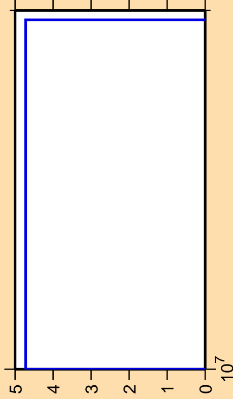
\Delta\sigma/\sigma vs. E for ^{248}\text{Cf}(n,\text{He3})
