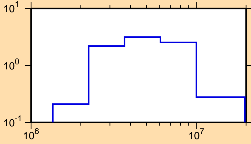
\sigma vs. E for ^{248}\text{Cf}(n,n\text{cont.})
