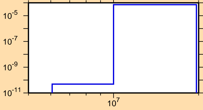
\sigma vs. E for ^{248}\text{Cf}(n,np)
