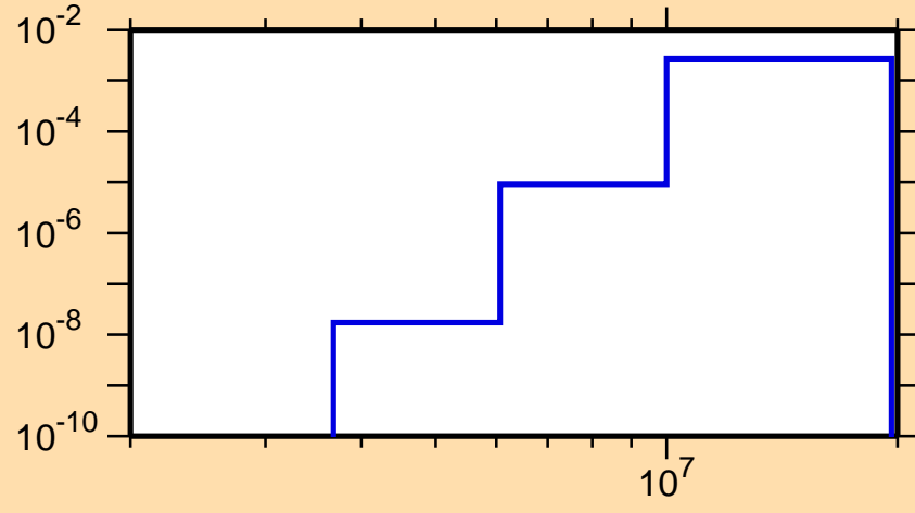
\sigma vs. E for ^{249}\text{Cf}(n,p)
