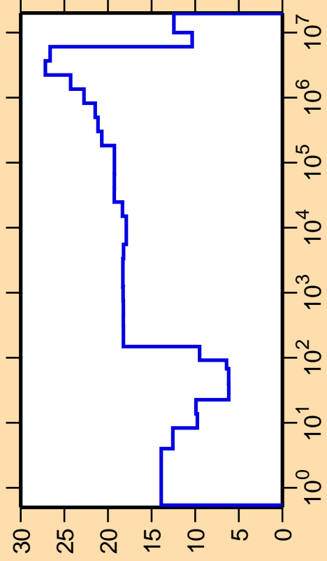
\Delta\sigma/\sigma vs. E for ^{249}\text{Cf}(n,\gamma)
