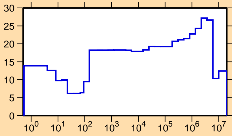
\Delta\sigma/\sigma vs. E for ^{249}\text{Cf}(n,\gamma)
