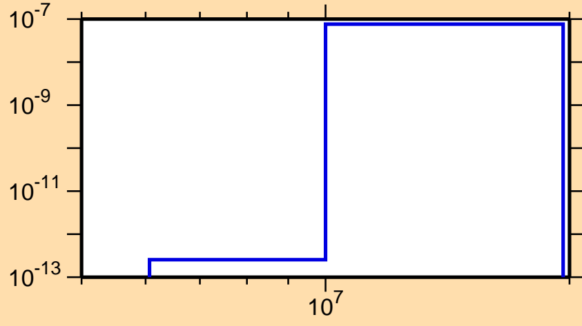
\sigma vs. E for ^{249}\text{Cf}(n,2n\alpha)
