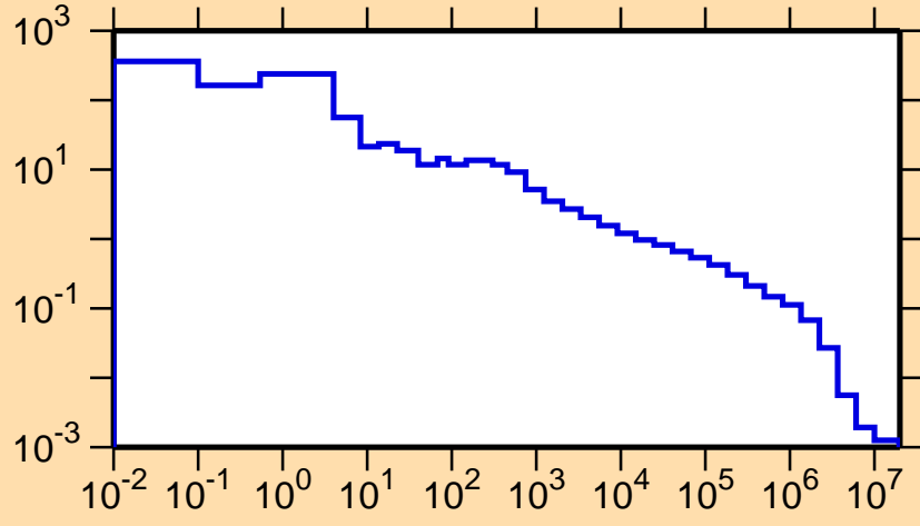
\sigma vs. E for ^{249}\text{Cf}(n,\gamma)
