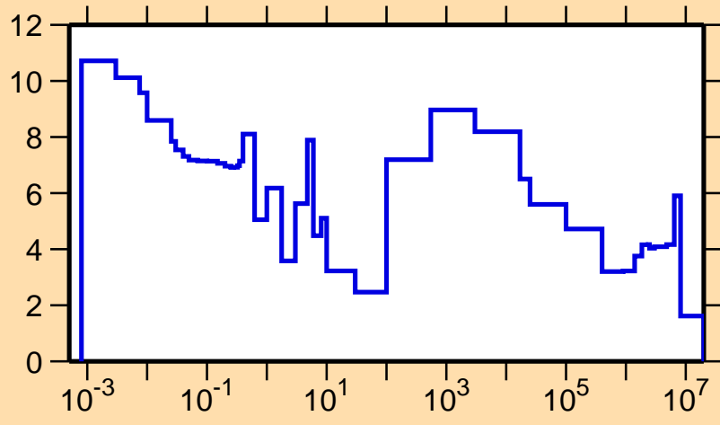
\Delta\sigma/\sigma vs. E for ^{249}\text{Cf}(n,f)
