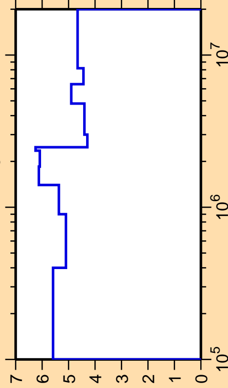
\Delta\sigma/\sigma vs. E for ^{249}\text{Cf}(n,n_3)
