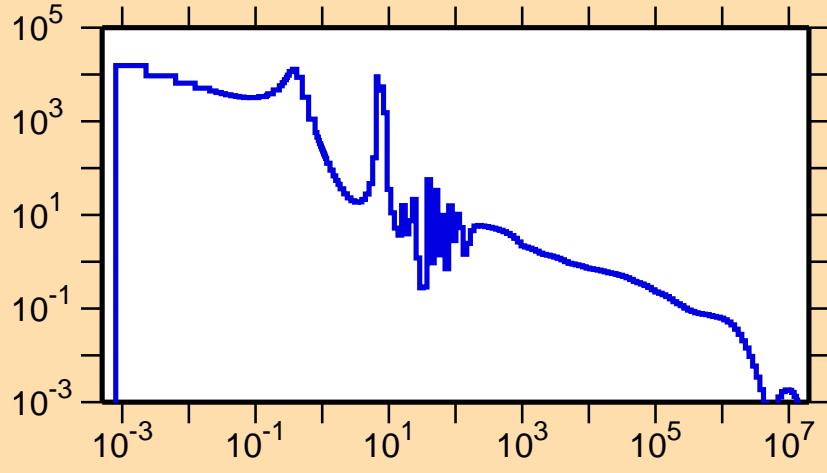
\sigma vs. E for ^{251}\text{Cf}(n,\gamma)
