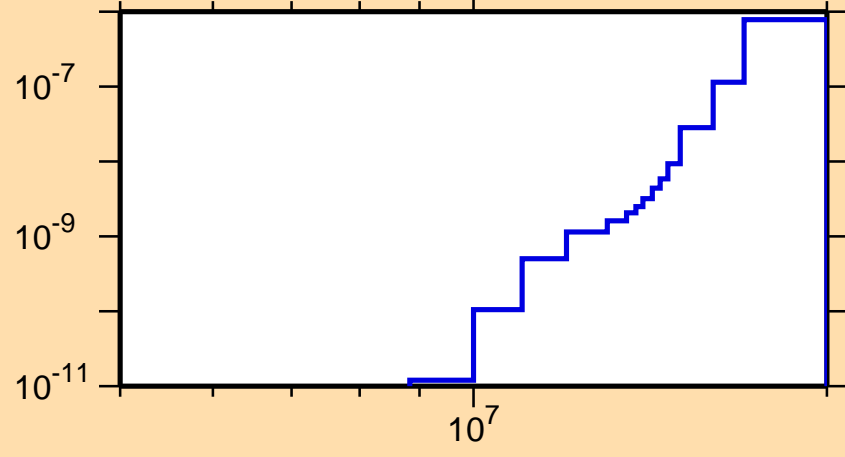
\sigma vs. E for ^{251}\text{Cf}(n,2n\alpha)
