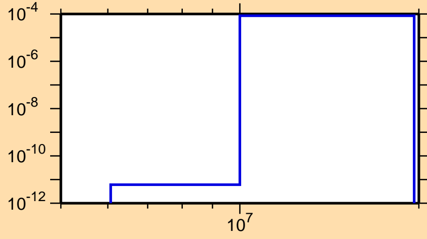
\sigma vs. E for ^{251}\text{Cf}(n,d)
