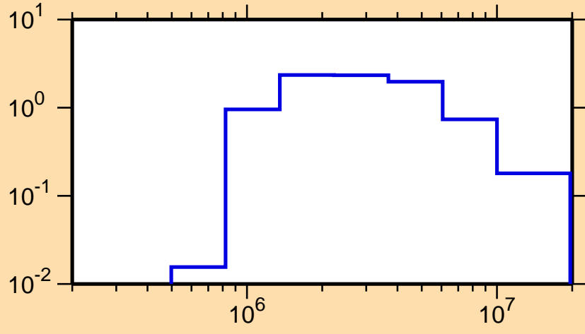
\sigma vs. E for ^{251}\text{Cf}(n,n\text{cont.})
