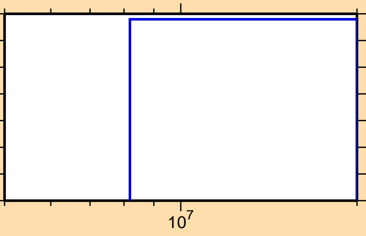
\sigma vs. E for ^{251}\text{Cf}(n,d)
