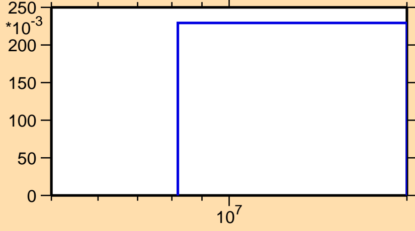
\sigma vs. E for ^{251}\text{Cf}(n,3n)
