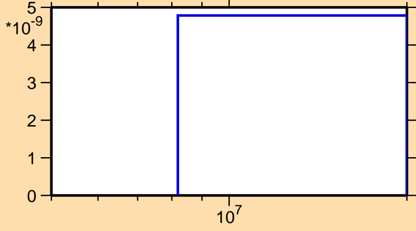
\sigma vs. E for ^{251}\text{Cf}(n,2np)
