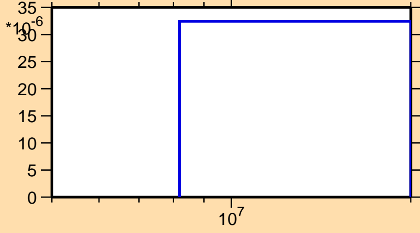
\sigma vs. E for ^{251}\text{Cf}(n,np)
