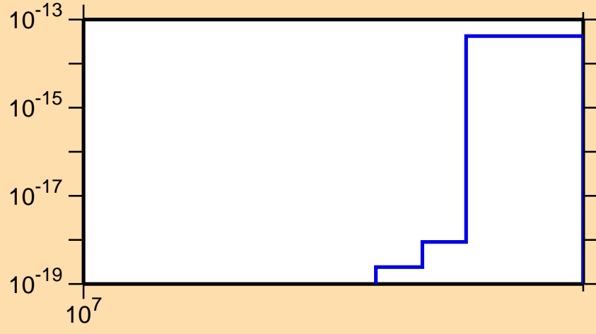
\sigma vs. E for ^{252}\text{Cf}(\text{mt } 11)
