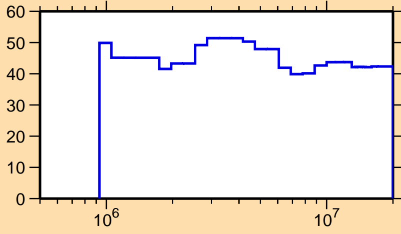
\Delta\sigma/\sigma vs. E for ^{252}\text{Cf}(n,incl.)
