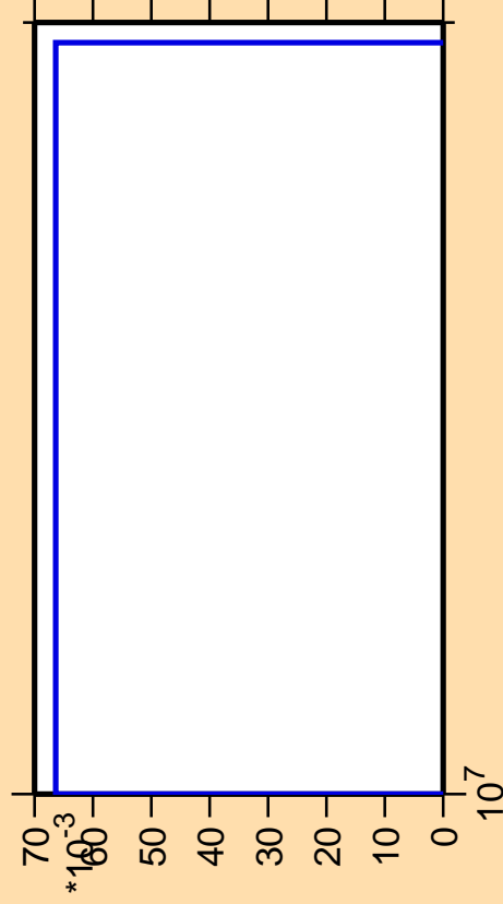
\Delta\sigma/\sigma vs. E for ^{252}\text{Cf}(n,\text{He3})
