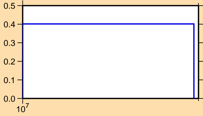
\sigma vs. E for ^{252}\text{Cf}(n,3n)
