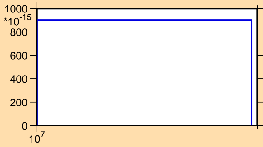
\sigma vs. E for ^{252}\text{Cf}(n,3n\alpha)
