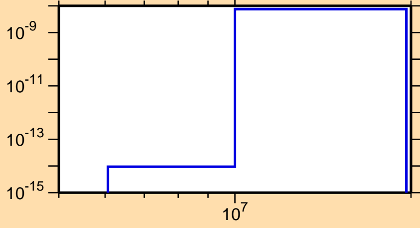
\sigma vs. E for ^{252}\text{Cf}(n,2n\alpha)
