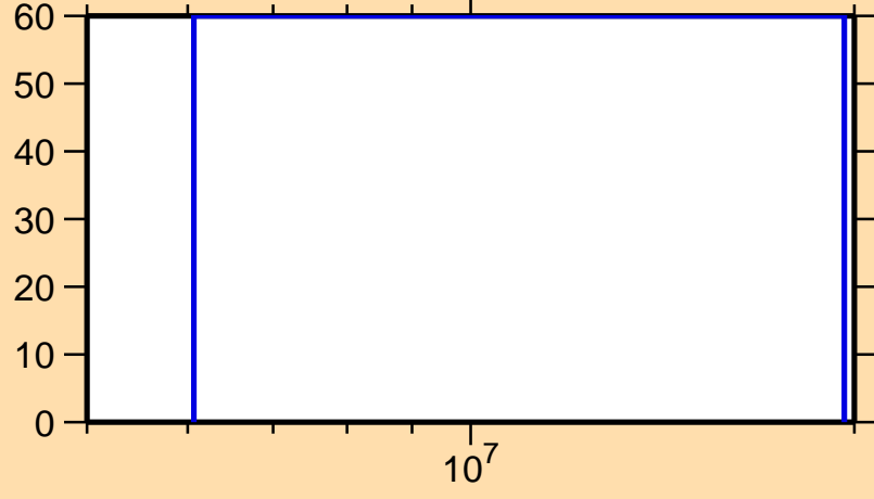
\Delta\sigma/\sigma vs. E for ^{252}\text{Cf}(n,2n)
