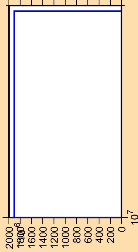
\Delta\sigma/\sigma vs. E for ^{252}\text{Cf}(\text{mt 11})
