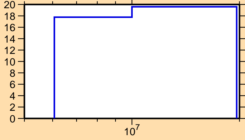
\Delta\sigma/\sigma vs. E for ^{252}\text{Cf}(n,\text{el.})
