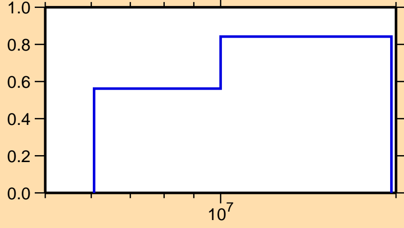
\sigma vs. E for ^{252}\text{Cf}(n,2n)
