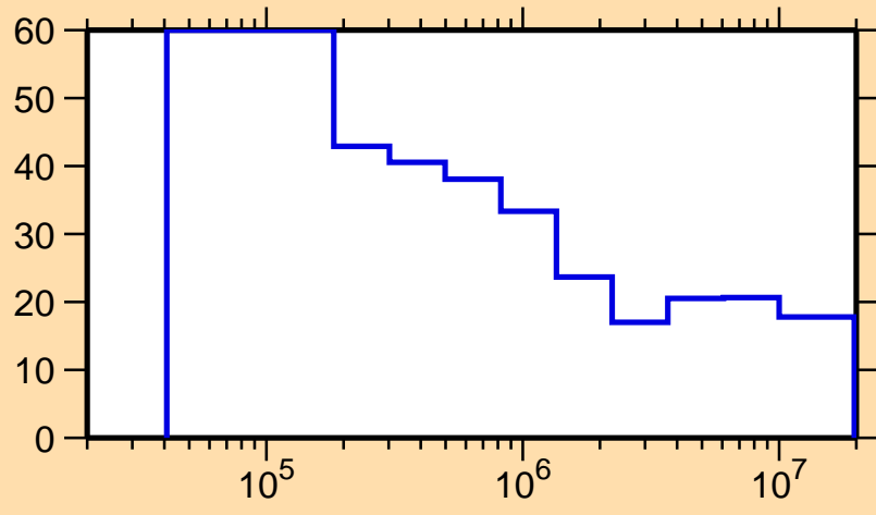
\Delta\sigma/\sigma vs. E for ^{252}\text{Cf}(n,\text{nonel.})
