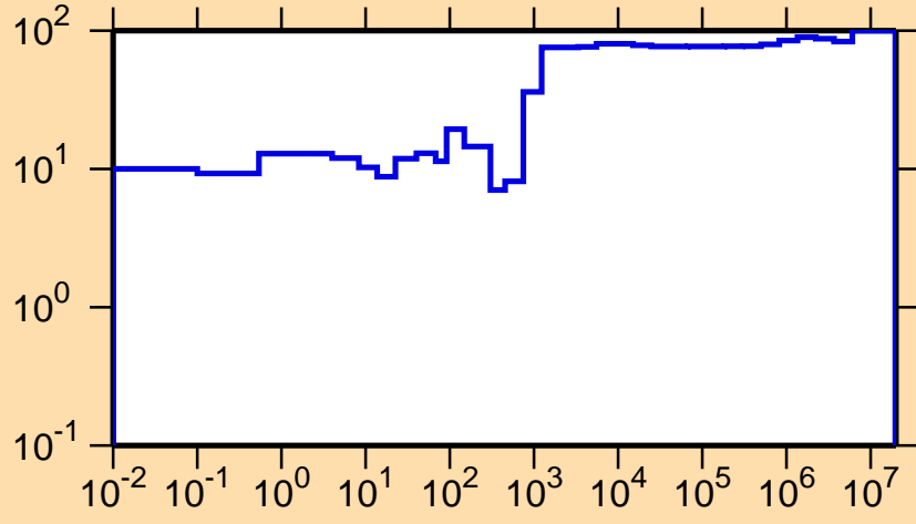
\Delta\sigma/\sigma vs. E for ^{252}\text{Cf}(n,\gamma)
