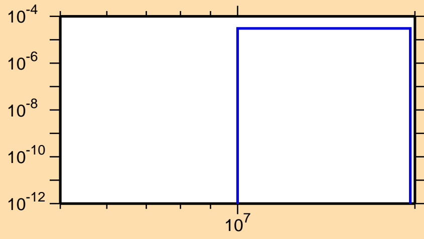
\sigma vs. E for ^{252}\text{Cf}(n,d)
