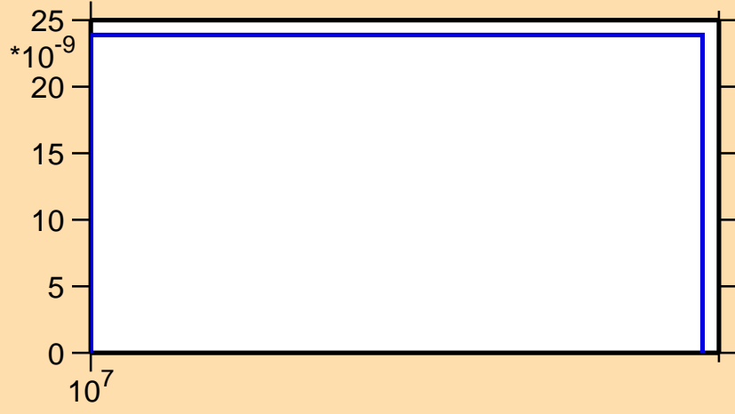
\sigma vs. E for ^{252}\text{Cf}(n,nt)
