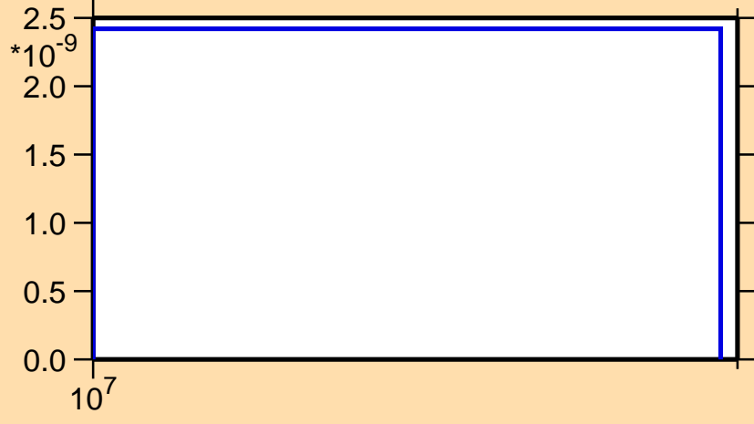
\sigma vs. E for ^{252}\text{Cf}(n,nd)
