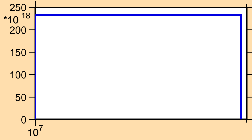
\sigma vs. E for ^{252}\text{Cf}(\text{mt 11})
