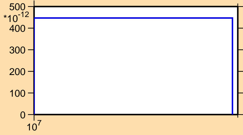
\sigma vs. E for ^{252}\text{Cf}(n,2np)
