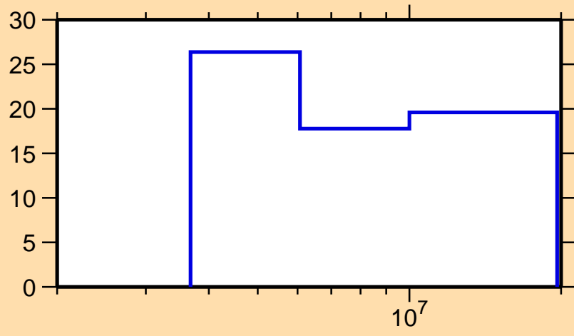
\Delta\sigma/\sigma vs. E for ^{252}\text{Cf}(n,el.)
