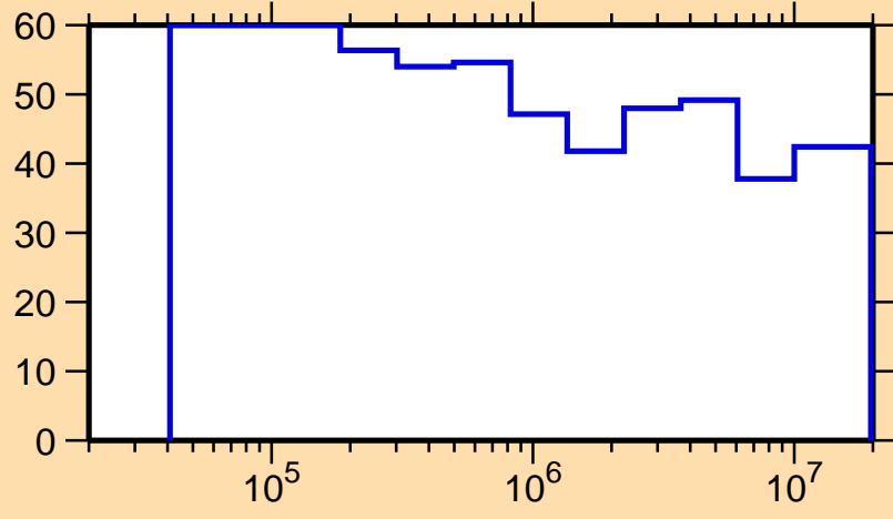
\Delta\sigma/\sigma vs. E for ^{252}\text{Cf}(n,\text{inel.})
