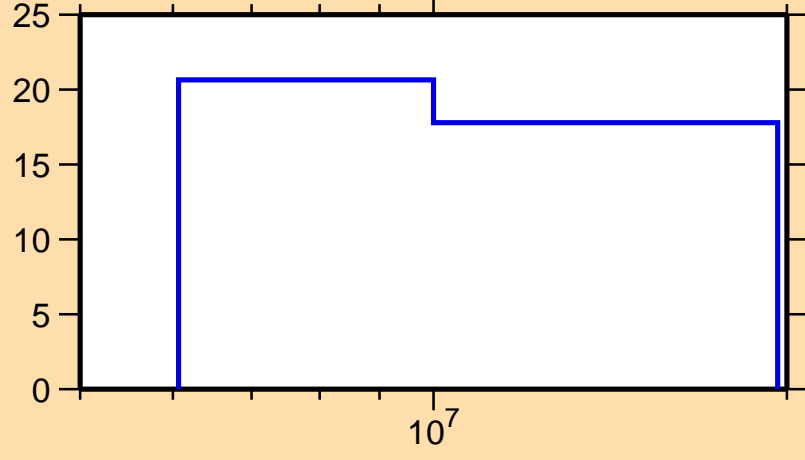
\Delta\sigma/\sigma vs. E for ^{252}\text{Cf}(n,\text{nonel.})
