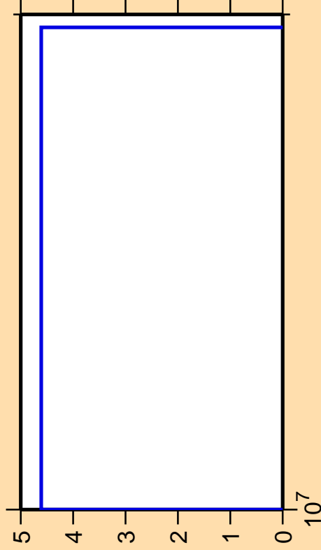
\Delta\sigma/\sigma vs. E for ^{252}\text{Cf}(n,3n\alpha)
