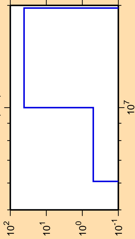
\Delta\sigma/\sigma vs. E for ^{252}\text{Cf}(n,d)
