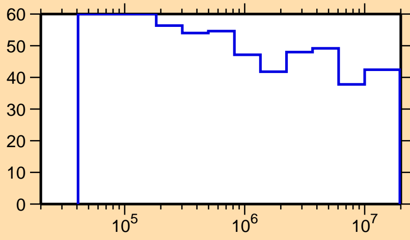
\Delta\sigma/\sigma vs. E for ^{252}\text{Cf}(n,\text{inel.})
