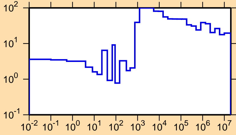
\Delta\sigma/\sigma vs. E for ^{252}\text{Cf}(n,el.)
