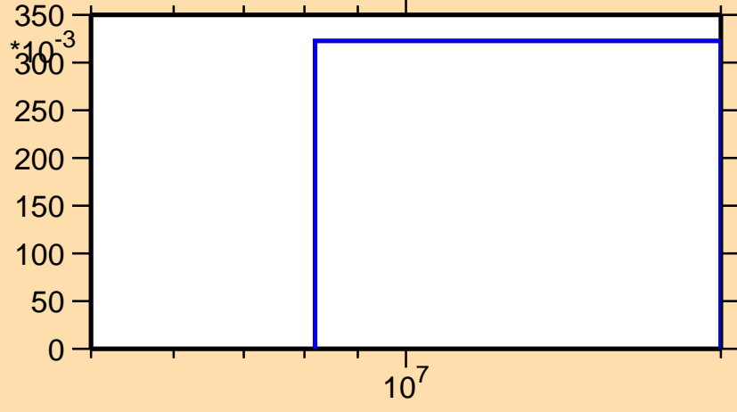
\sigma vs. E for ^{252}\text{Cf}(n,3n)
