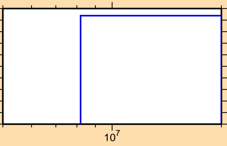
\sigma vs. E for ^{252}\text{Cf}(n,t)
