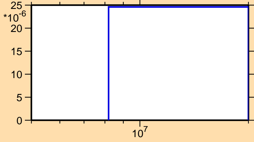
\sigma vs. E for ^{252}\text{Cf}(n,d)
