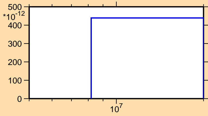
\sigma vs. E for ^{252}\text{Cf}(n,2np)
