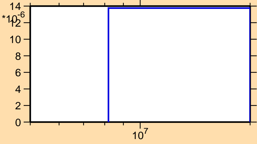
\sigma vs. E for ^{252}\text{Cf}(n,np)
