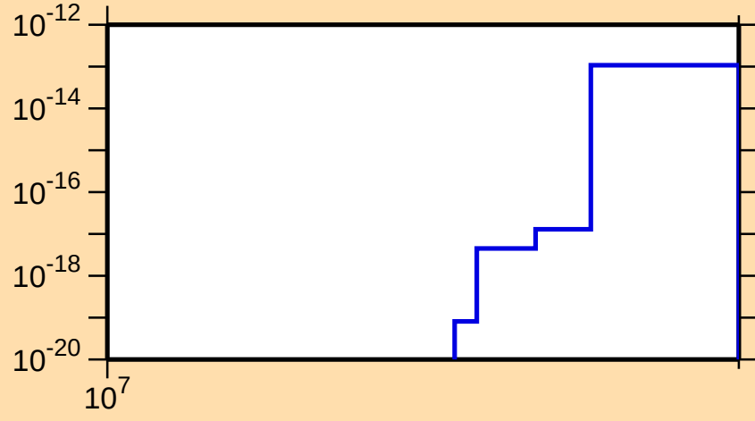
\sigma vs. E for ^{253}\text{Cf}(\text{mt 11})
