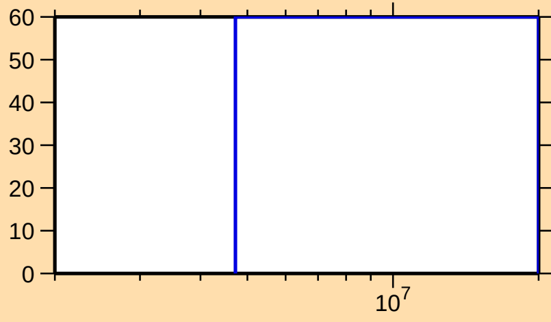
\Delta\sigma/\sigma vs. E for ^{253}\text{Cf}(n,2n)
