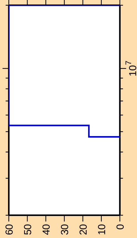
\Delta\sigma/\sigma vs. E for ^{253}\text{Cf}(n,p)
