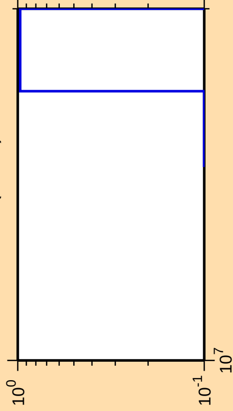
\Delta\sigma/\sigma vs. E for ^{253}\text{Cf}(\text{mt 11})
