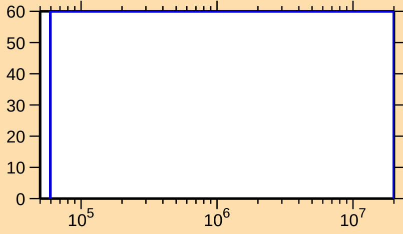
\Delta\sigma/\sigma vs. E for ^{253}\text{Cf}(n,\text{inel.})
