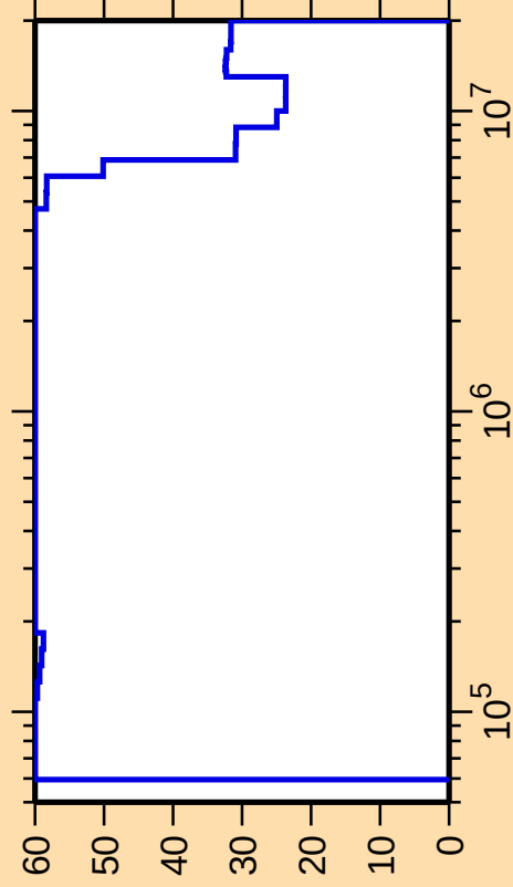
\Delta\sigma/\sigma vs. E for ^{253}\text{Cf}(n,f)
