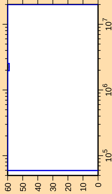
\Delta\sigma/\sigma vs. E for ^{253}\text{Cf}(n,n_1)
