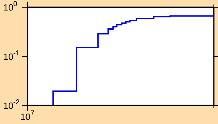
\sigma vs. E for ^{253}\text{Cf}(n,3n)
