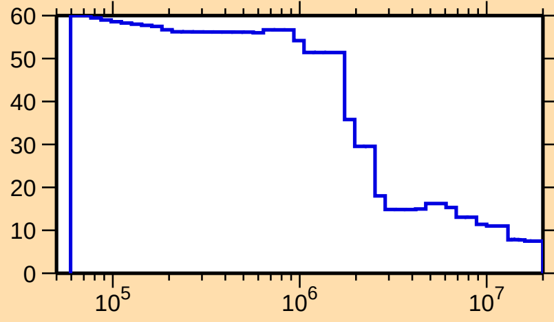
\Delta\sigma/\sigma vs. E for ^{253}\text{Cf}(n,\text{nonel.})
