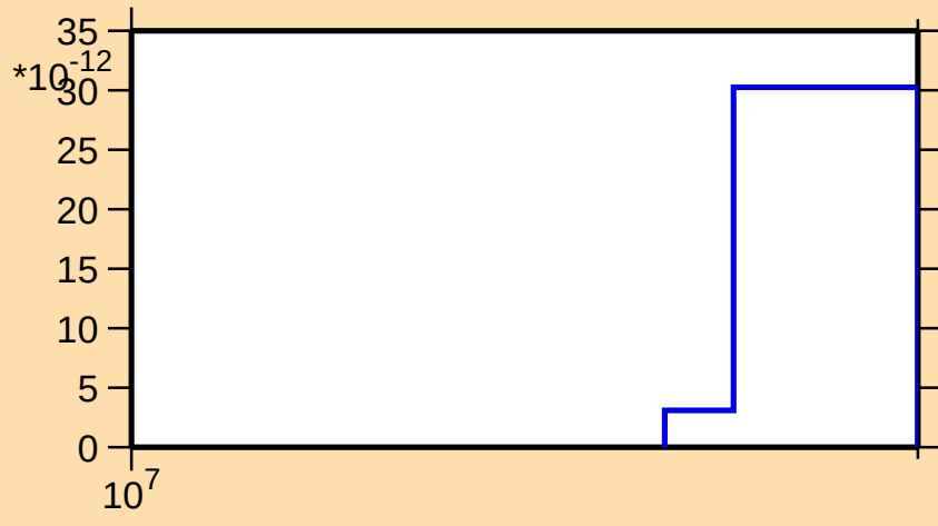
\sigma vs. E for ^{253}\text{Cf}(n,3n\alpha)
