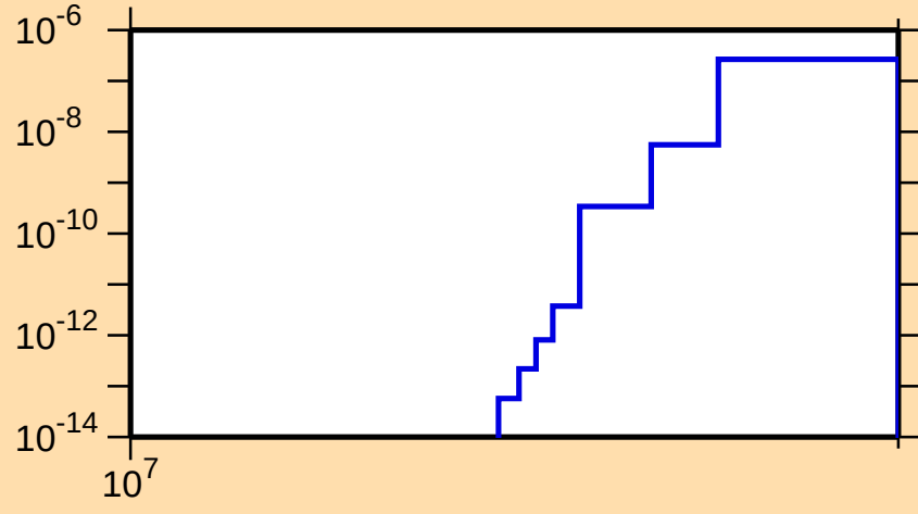
\sigma vs. E for ^{253}\text{Cf}(n,2np)
