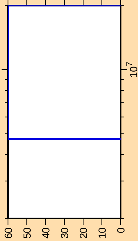
\Delta\sigma/\sigma vs. E for ^{253}\text{Cf}(n,n\text{cont.})
