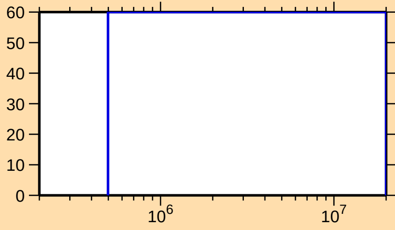
\Delta\sigma/\sigma vs. E for ^{253}\text{Cf}(n,n\text{cont.})
