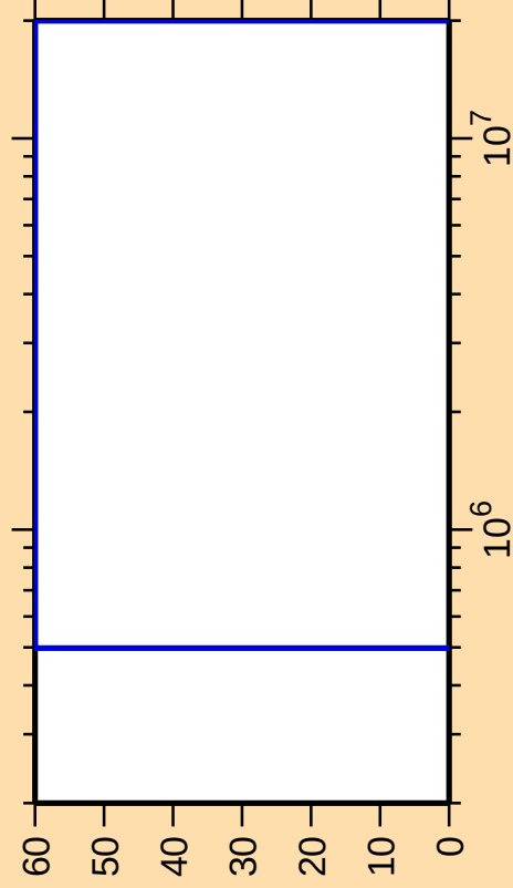
\Delta\sigma/\sigma vs. E for ^{253}\text{Cf}(n,\text{ncont.})
