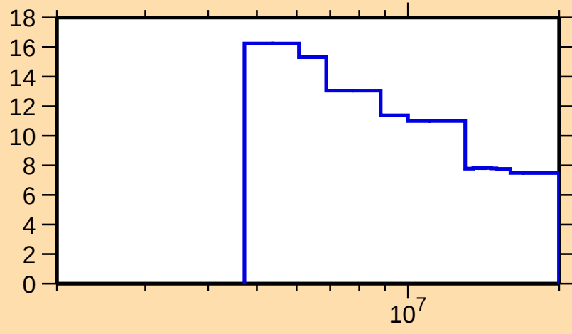
\Delta\sigma/\sigma vs. E for ^{253}\text{Cf}(n,\text{nonel.})
