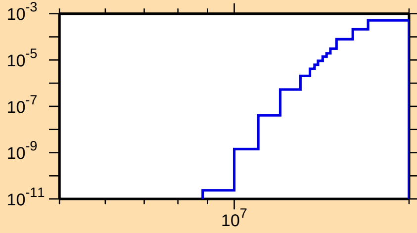
\sigma vs. E for ^{253}\text{Cf}(n,t)
