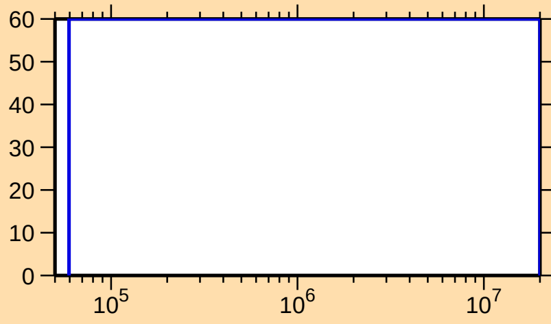
\Delta\sigma/\sigma vs. E for ^{253}\text{Cf}(n,\text{inel.})
