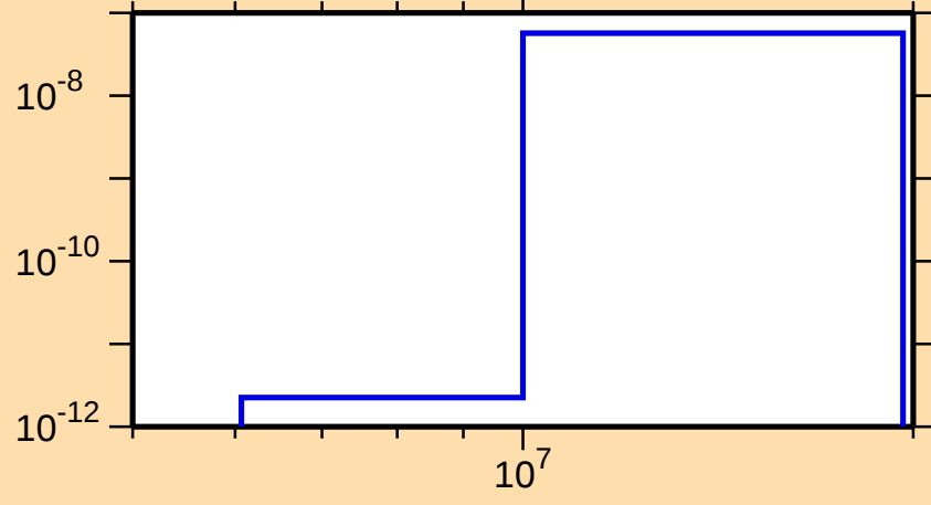
\sigma vs. E for ^{253}\text{Cf}(n,2n\alpha)
