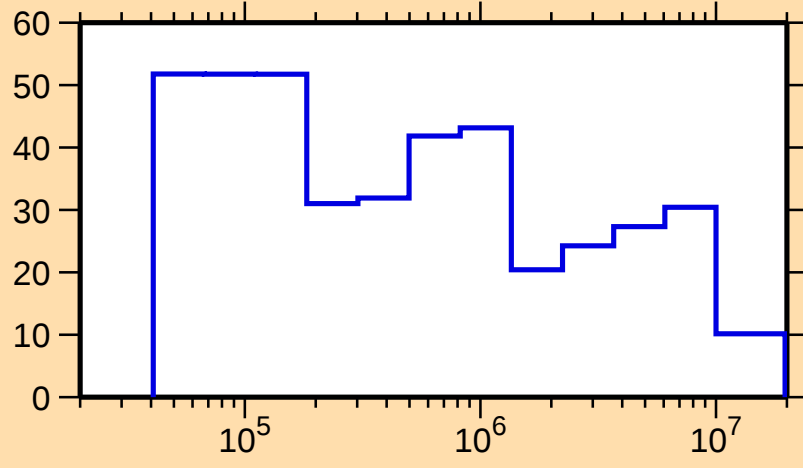
\Delta\sigma/\sigma vs. E for ^{253}\text{Cf}(n,\text{el.})
