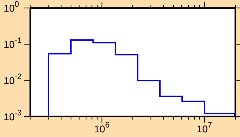
\sigma vs. E for ^{253}\text{Cf}(n,n_4)
