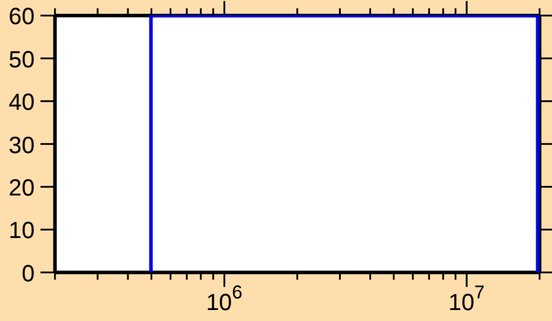
\Delta\sigma/\sigma vs. E for ^{253}\text{Cf}(n,n\text{cont.})
