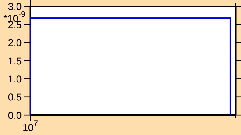
\sigma vs. E for ^{253}\text{Cf}(n,2np)
