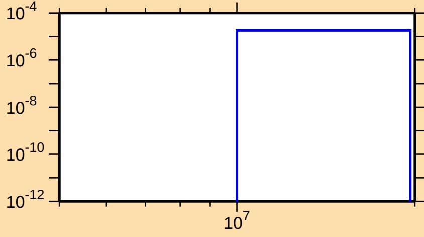
\sigma vs. E for ^{253}\text{Cf}(n,np)
