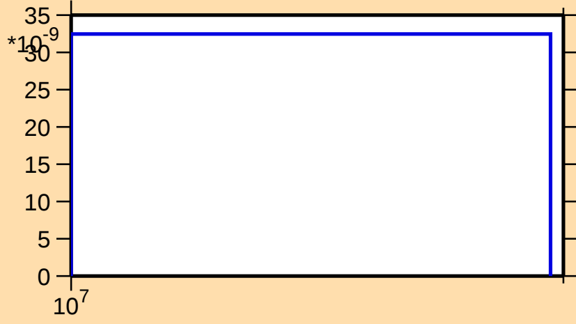
\sigma vs. E for ^{253}\text{Cf}(n,nt)
