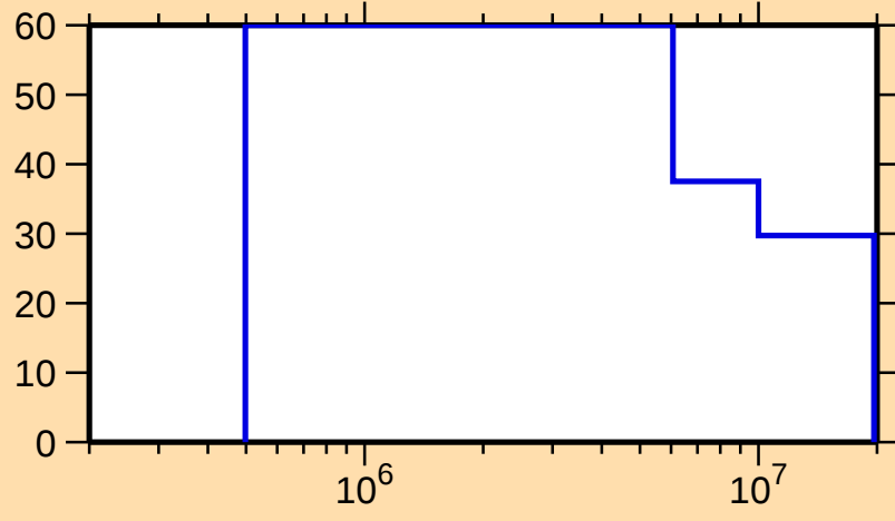
\Delta\sigma/\sigma vs. E for ^{253}\text{Cf}(n,f)
