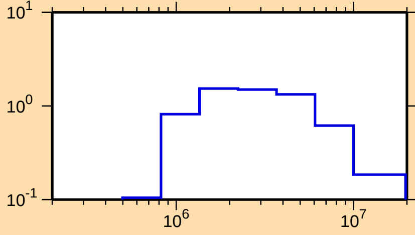
\sigma vs. E for ^{253}\text{Cf}(n,n\text{cont.})
