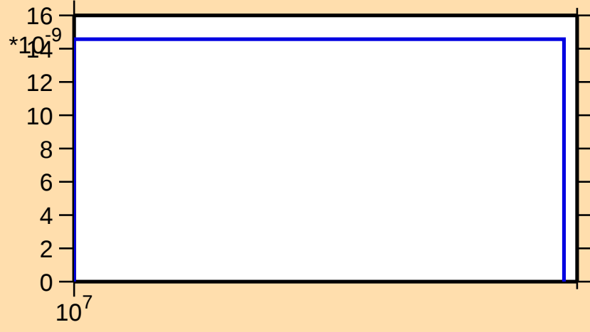
\sigma vs. E for ^{253}\text{Cf}(n,\text{nd})
