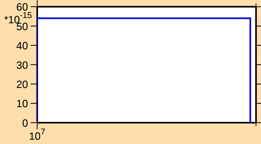
\sigma vs. E for ^{253}\text{Cf}(n,\text{He3})
