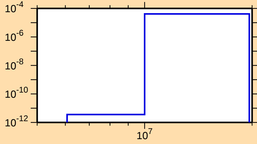
\sigma vs. E for ^{253}\text{Cf}(n,d)
