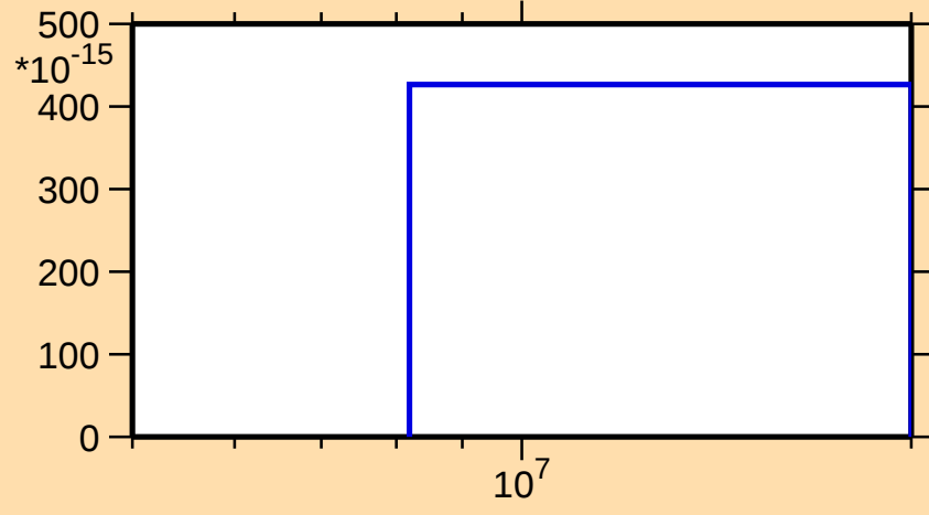
\sigma vs. E for ^{253}\text{Cf}(n,3n\alpha)
