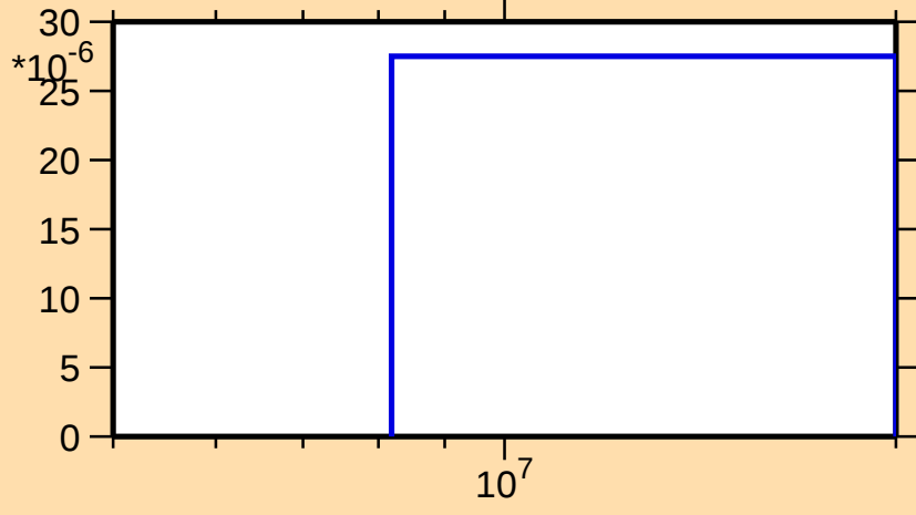
\sigma vs. E for ^{253}\text{Cf}(n,t)
