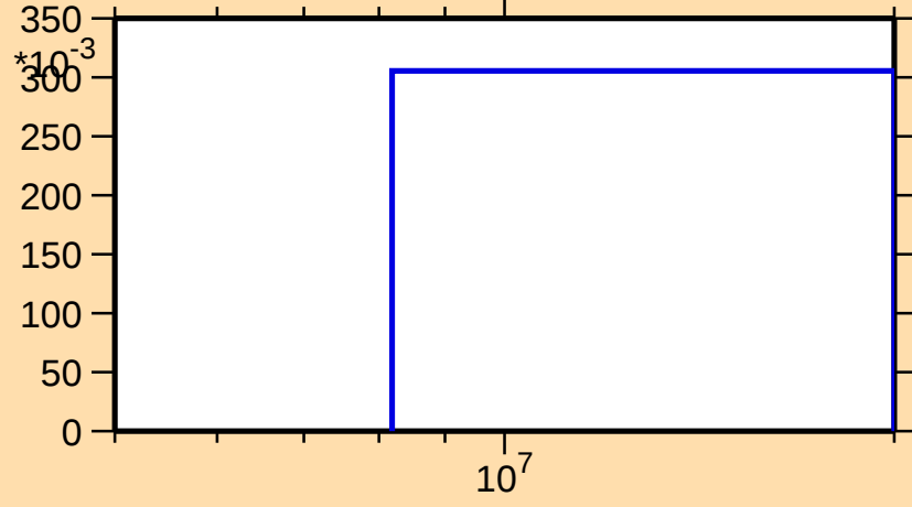
\sigma vs. E for ^{253}\text{Cf}(n,3n)
