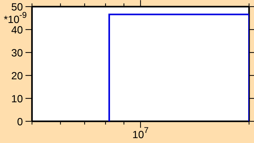
\sigma vs. E for ^{253}\text{Cf}(n,2n\alpha)
