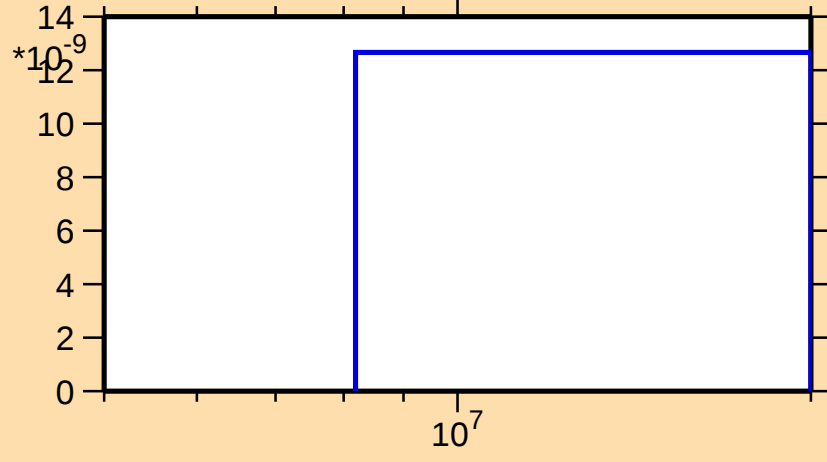
\sigma vs. E for ^{253}\text{Cf}(n,nd)
