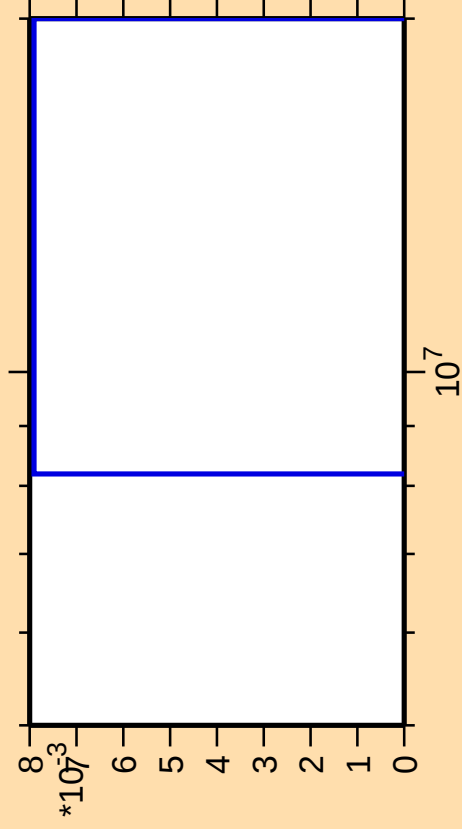
\Delta\sigma/\sigma vs. E for ^{253}\text{Cf}(\text{mt } 11)
