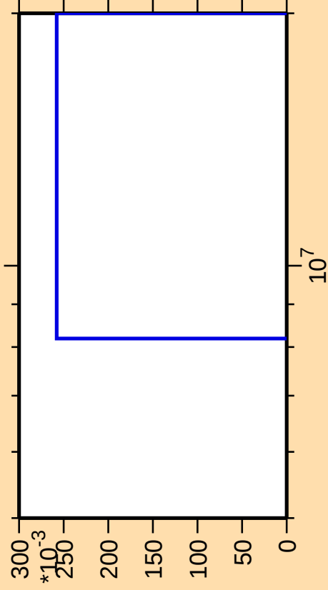
\Delta\sigma/\sigma vs. E for ^{253}\text{Cf}(n,\text{He3})
