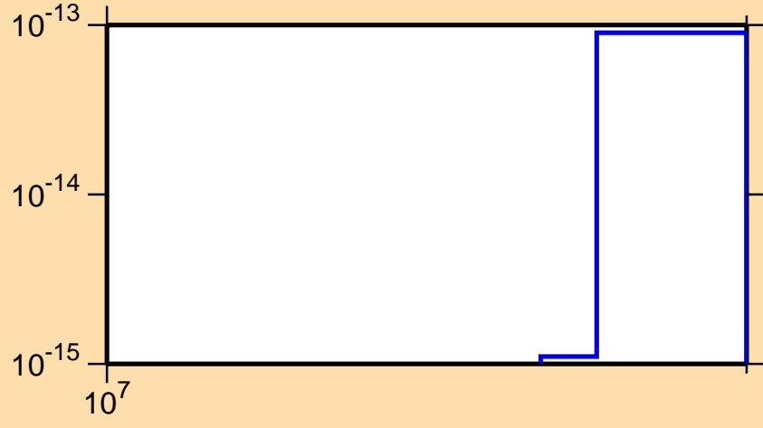
\sigma vs. E for ^{256}\text{Cf}(n,\text{He3})
