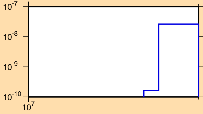
\sigma vs. E for ^{256}\text{Cf}(n,2np)
