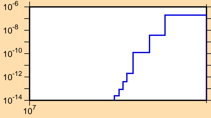
\sigma vs. E for ^{256}\text{Cf}(n,nd)
