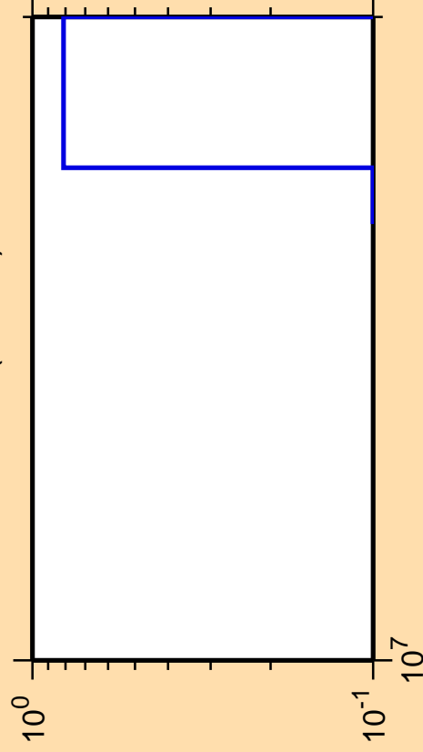
\Delta\sigma/\sigma vs. E for ^{256}\text{Cf}(n,\text{He3})
