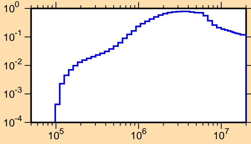
\sigma vs. E for ^{256}\text{Cf}(n,n\text{cont.})
