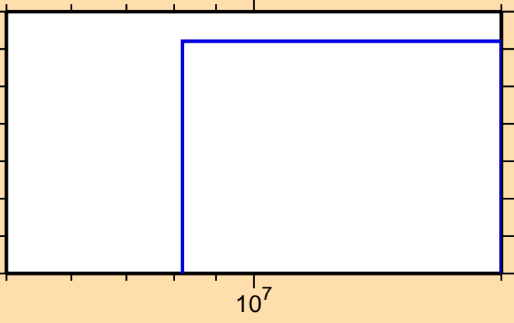
\sigma vs. E for ^{256}\text{Cf}(n,3n)
