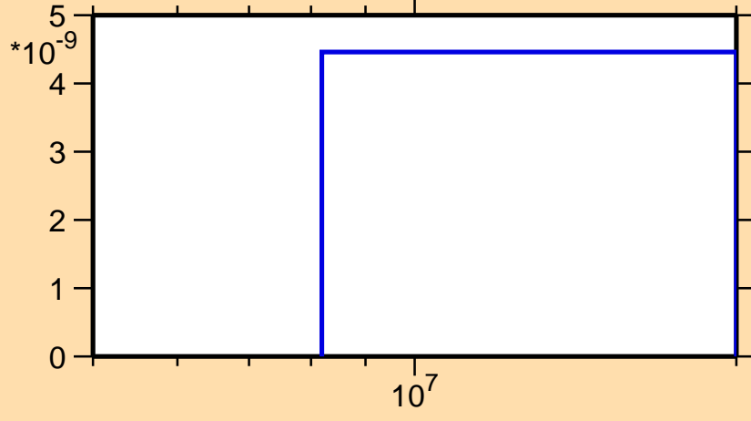
\sigma vs. E for ^{256}\text{Cf}(n,2n\alpha)
