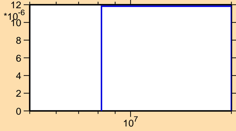
\sigma vs. E for ^{256}\text{Cf}(n,d)
