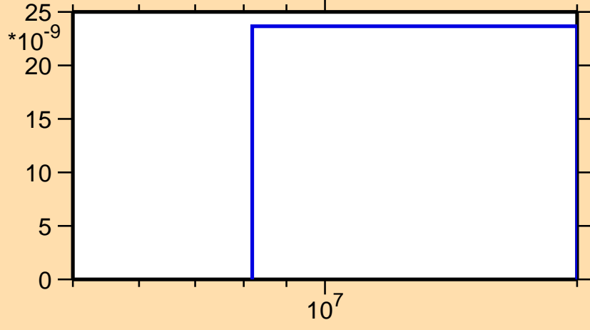
\sigma vs. E for ^{256}\text{Cf}(n,nt)
