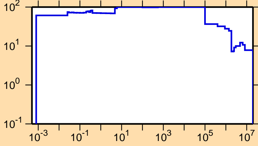
\Delta\sigma/\sigma vs. E for ^{256}\text{Cf}(n,\text{nonel.})
