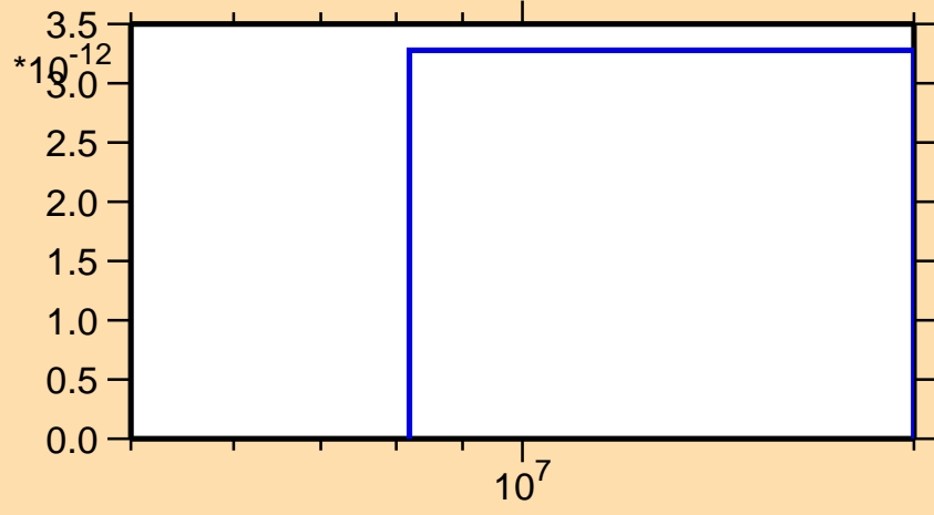
\sigma vs. E for ^{256}\text{Cf}(n,3n\alpha)
