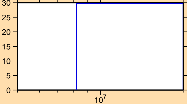
\Delta\sigma/\sigma vs. E for ^{33}\text{Cl}(n,2n)
