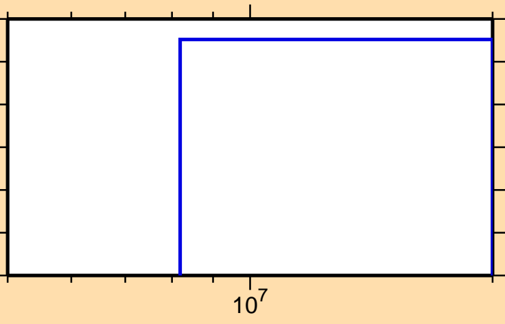
\sigma vs. E for ^{33}\text{Cl}(n,2np)
