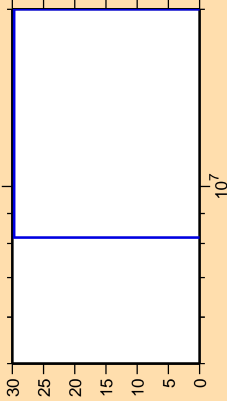
\Delta\sigma/\sigma vs. E for ^{33}\text{Cl}(n,2n)
