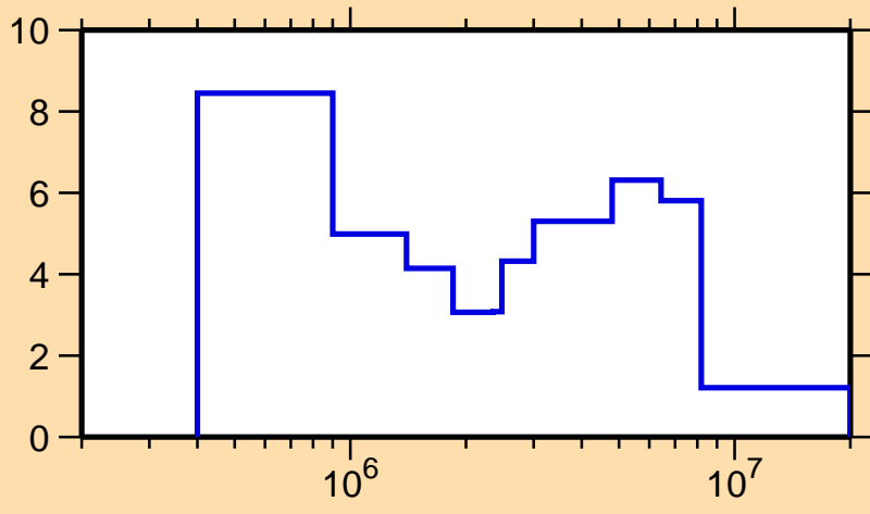
\Delta\sigma/\sigma vs. E for ^{33}\text{Cl}(n,\text{el.})
