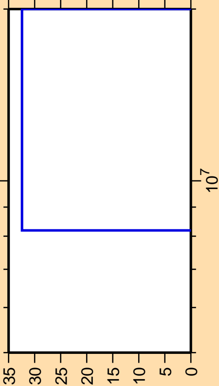
\Delta\sigma/\sigma vs. E for ^{33}\text{Cl}(n,\gamma)
