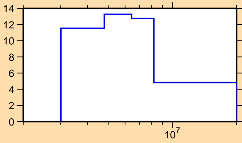
\Delta\sigma/\sigma vs. E for ^{34}\text{Cl}(n, el.)
