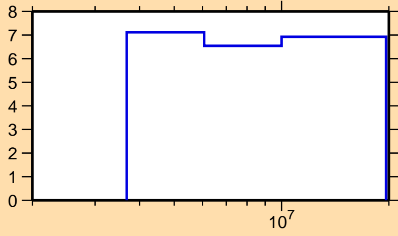
\Delta\sigma/\sigma vs. E for ^{35}\text{Cl}(n,n\text{onel.})
