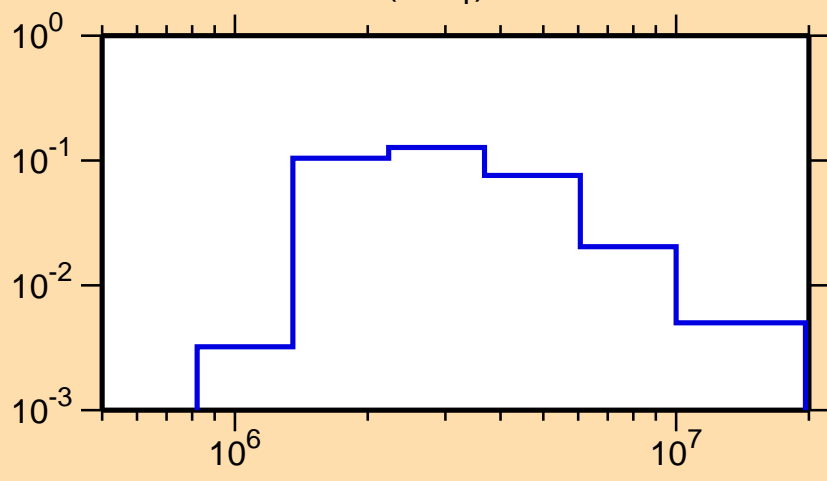
\sigma vs. E for ^{35}\text{Cl}(n,n_1)
