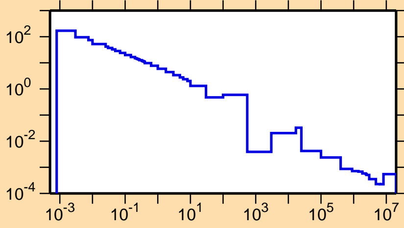
\sigma vs. E for ^{35}\text{Cl}(n,\gamma)
