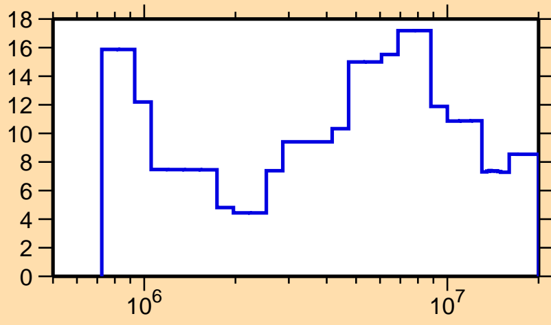
\Delta\sigma/\sigma vs. E for ^{36}\text{Cl}(n,\text{el.})
