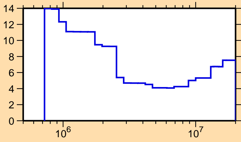
\Delta\sigma/\sigma vs. E for ^{36}\text{Cl}(n,\text{nonel.})
