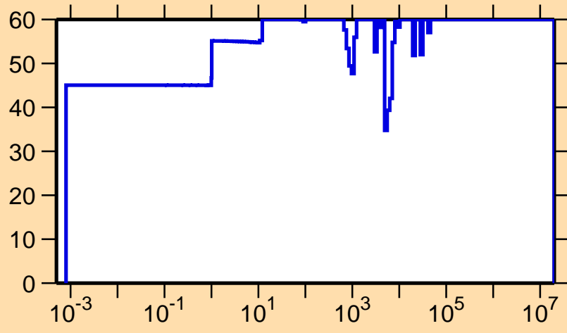
\Delta\sigma/\sigma vs. E for ^{36}\text{Cl}(n,\gamma)
