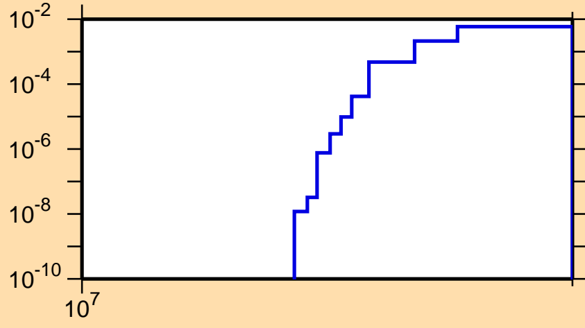
\sigma vs. E for ^{36}\text{Cl}(n,nd)
