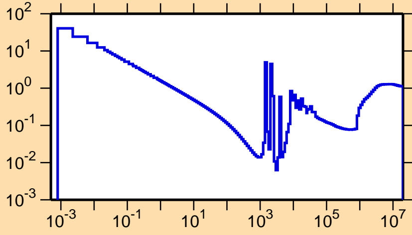
\sigma vs. E for ^{36}\text{Cl}(n,\text{nonel.})
