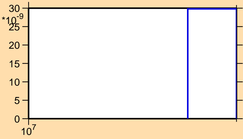
\sigma vs. E for ^{36}\text{Cl}(n,nt)
