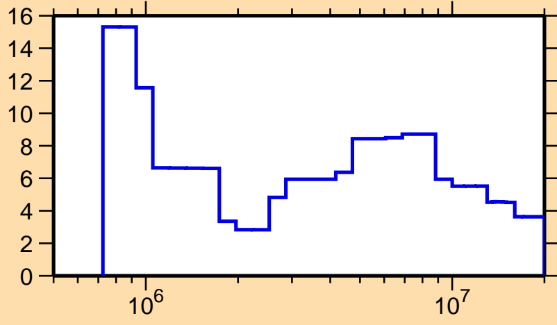
\Delta\sigma/\sigma vs. E for ^{36}\text{Cl}(n,\text{tot.})
