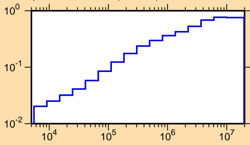
\mu vs. E for ^{36}\text{Cl}(\text{mt251})
