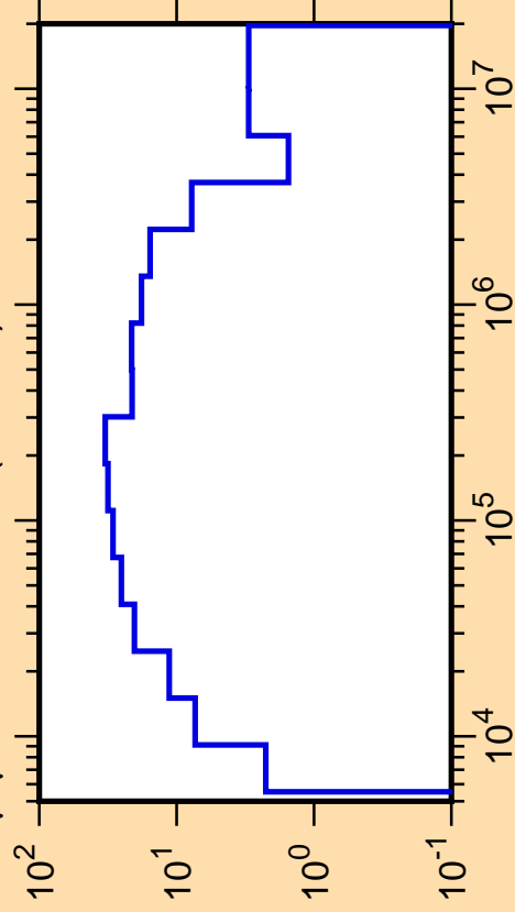
\Delta\mu/\mu vs. E for ^{36}\text{Cl}(\text{mt251})
