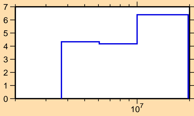
\Delta\sigma/\sigma vs. E for ^{36}\text{Cl}(n,n\text{onel.})
