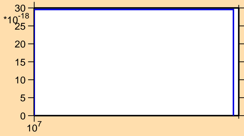
\sigma vs. E for ^{36}\text{Cl} (mt 34)
