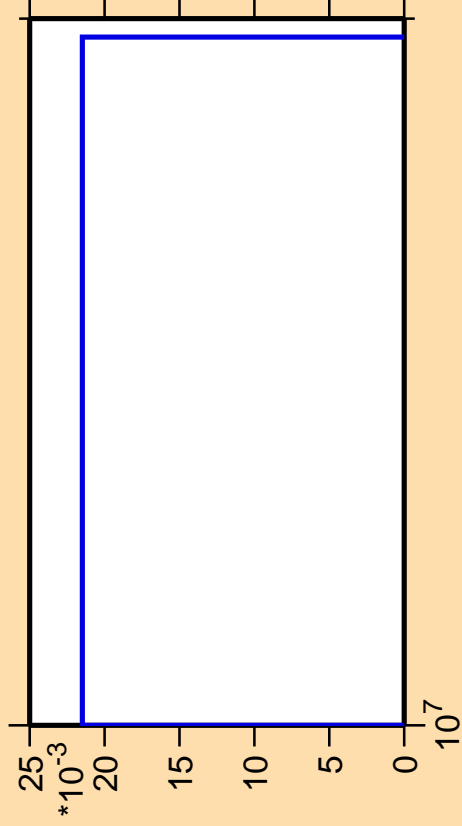
\Delta\sigma/\sigma vs. E for ^{36}\text{Cl}(n,\text{pd})
