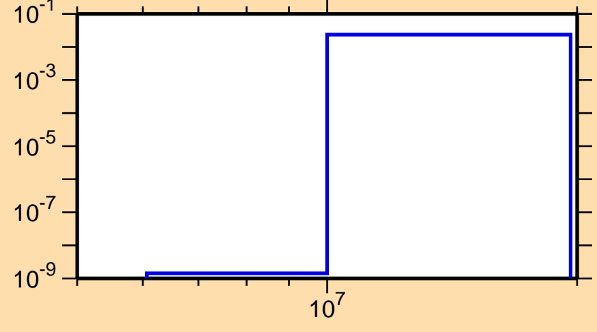
\sigma vs. E for ^{36}\text{Cl}(n,n\alpha)
