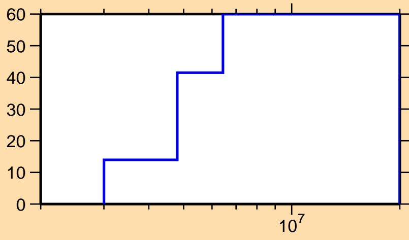
\Delta\sigma/\sigma vs. E for ^{36}\text{Cl}(n,n_1)
