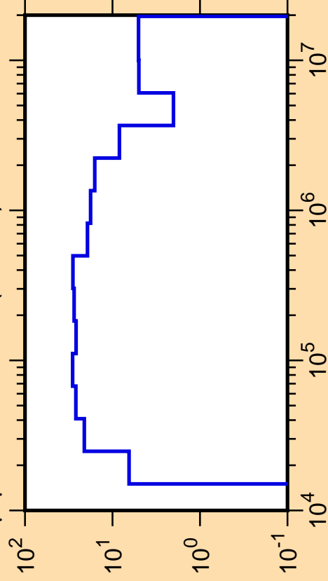
\Delta\mu/\mu vs. E for ^{37}\text{Cl}(\text{mt251})
