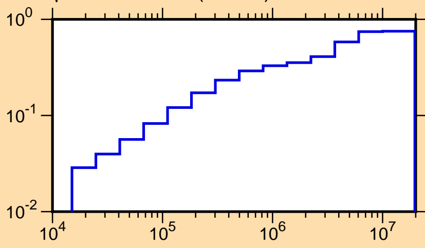
\mu vs. E for ^{37}\text{Cl}(\text{mt251})
