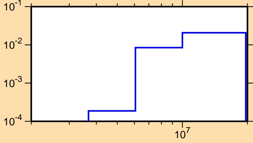
\sigma vs. E for ^{37}\text{Cl}(n,p)
