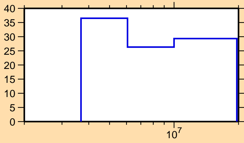
\Delta\sigma/\sigma vs. E for ^{37}\text{Cl}(n,p)
