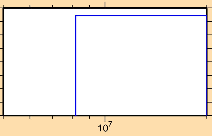
\sigma vs. E for ^{37}\text{Cl}(n,\text{He3})
