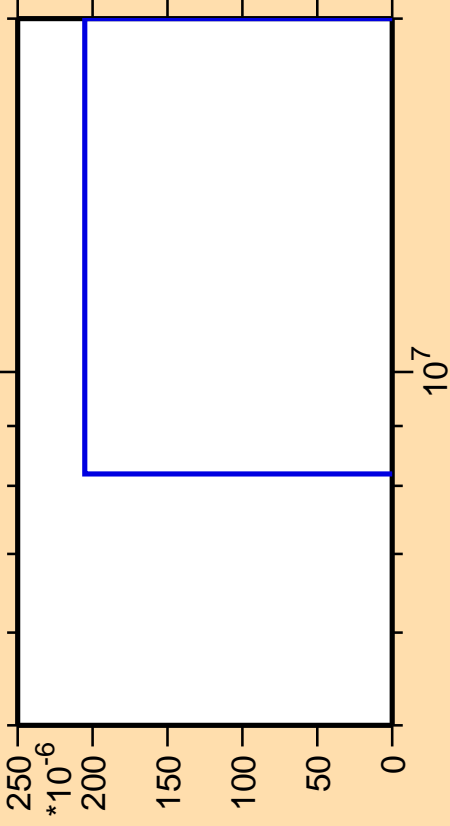
\Delta\sigma/\sigma vs. E for ^{37}\text{Cl}(n,2n\alpha)
