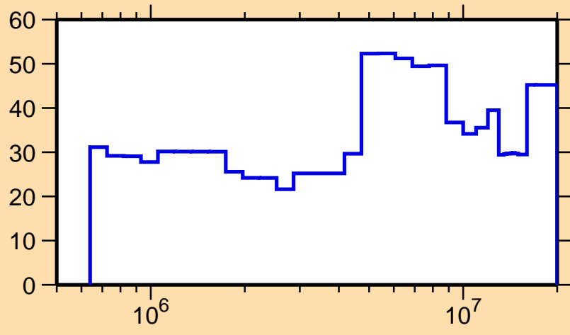
\Delta\sigma/\sigma vs. E for ^{38}\text{Cl}(n,n_1)
