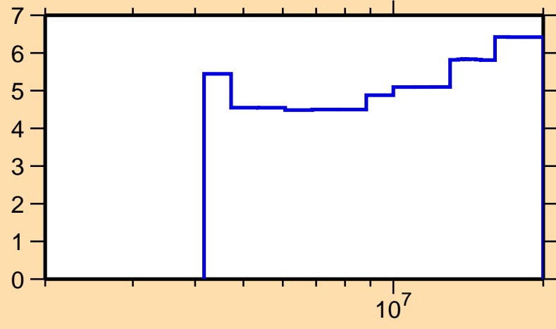
\Delta\sigma/\sigma vs. E for ^{38}\text{Cl}(n, n\text{onel.})
