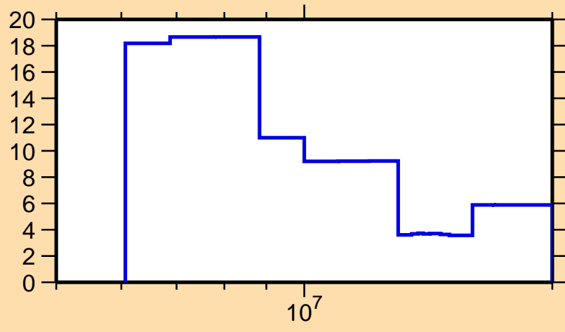
\Delta\sigma/\sigma vs. E for ^{38}\text{Cl}(n,\text{el.})
