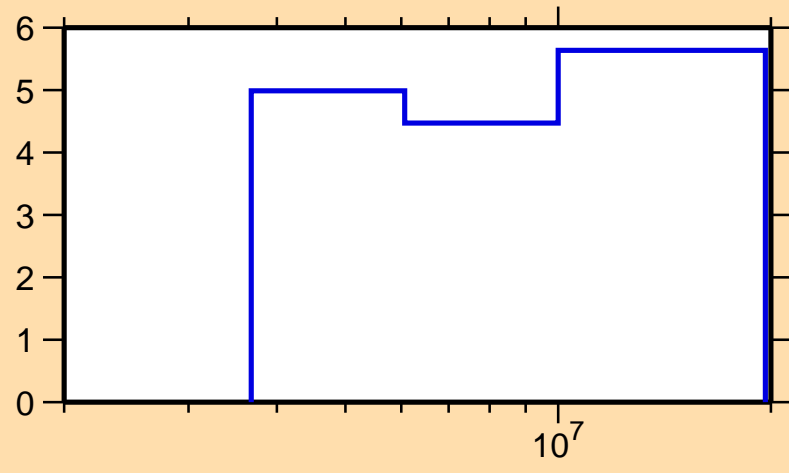
\Delta\sigma/\sigma vs. E for ^{38}\text{Cl}(n,n\text{nonel.})
