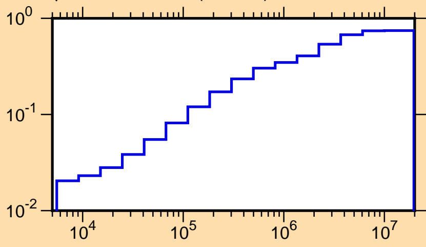
\mu vs. E for ^{39}\text{Cl}(\text{mt251})
