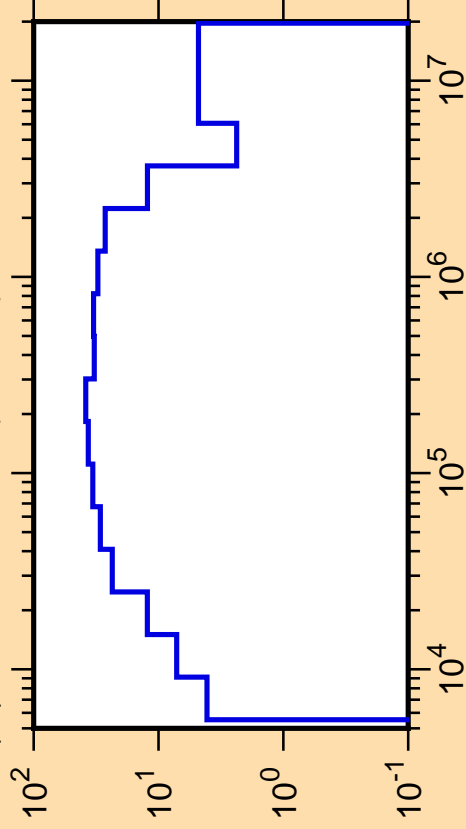
\Delta\mu/\mu vs. E for ^{39}\text{Cl}(\text{mt251})
