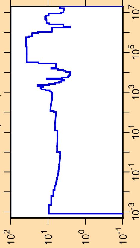
\Delta\sigma/\sigma vs. E for ^{40}\text{Cl}(n,\text{tot.})
