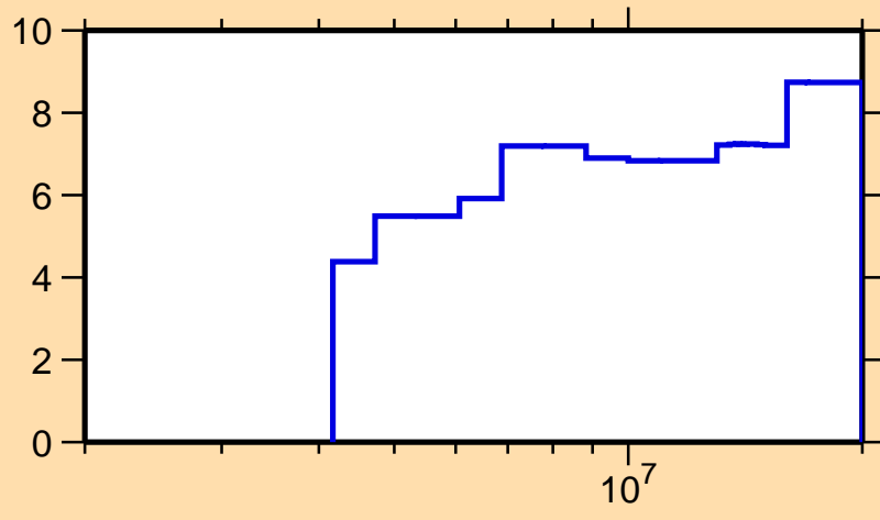
\Delta\sigma/\sigma vs. E for ^{40}\text{Cl}(n,n\text{nonel.})
