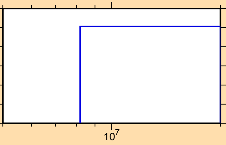
\sigma vs. E for ^{40}\text{Cl}(n,3n)
