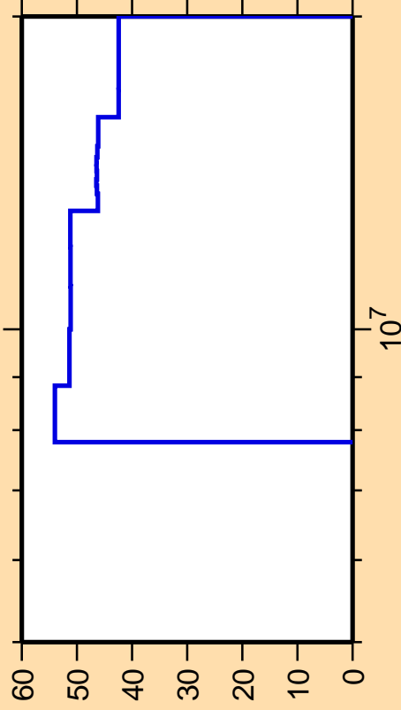
\Delta\sigma/\sigma vs. E for ^{41}\text{Cl}(n,n_1)
