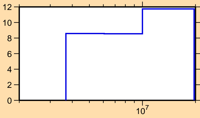
\Delta\sigma/\sigma vs. E for ^{41}\text{Cl}(n,n\text{nonel.})
