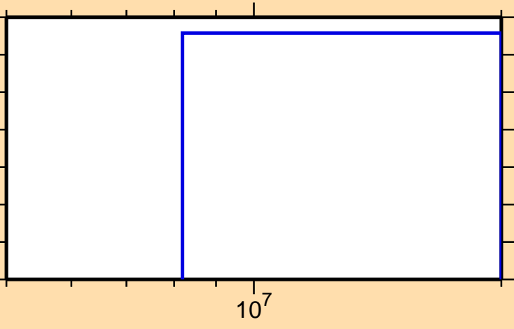
\sigma vs. E for ^{232}\text{Cm}(n,t)
