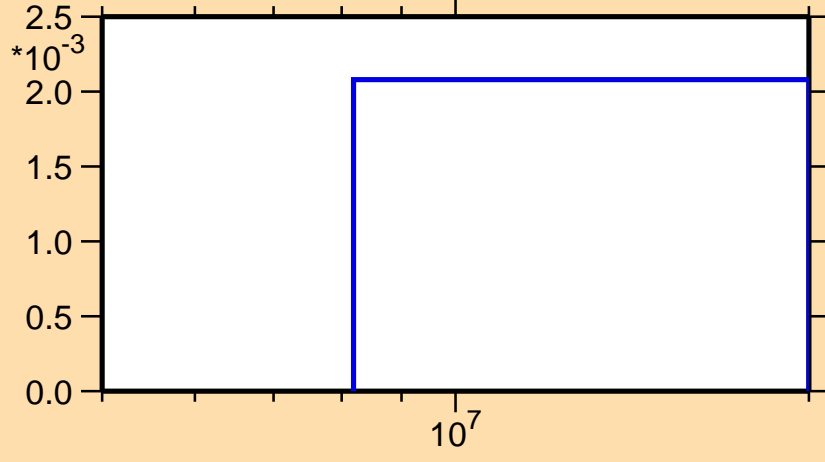
\sigma vs. E for ^{232}\text{Cm}(n,2n)
