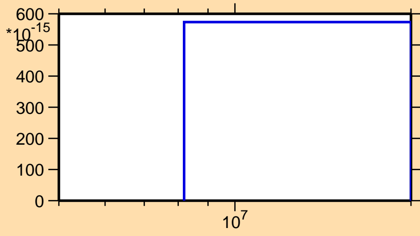
\sigma vs. E for ^{232}\text{Cm}(\text{mt117})
