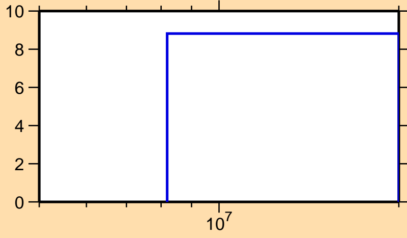
\Delta\sigma/\sigma vs. E for ^{232}\text{Cm}(n,\text{nonel.})
