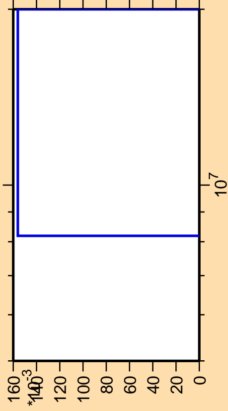
\Delta\sigma/\sigma vs. E for ^{232}\text{Cm} (mt 45)
