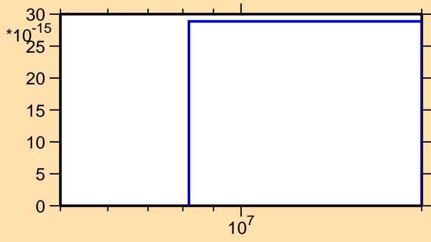
\sigma vs. E for ^{232}\text{Cm} (mt 45)
