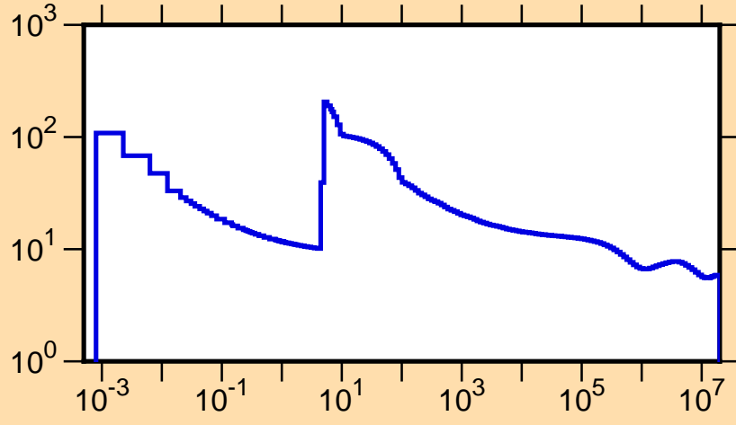
\sigma vs. E for ^{233}\text{Cm}(n,\text{tot.})
