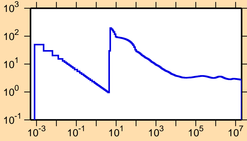
\sigma vs. E for ^{233}\text{Cm}(n,f)
