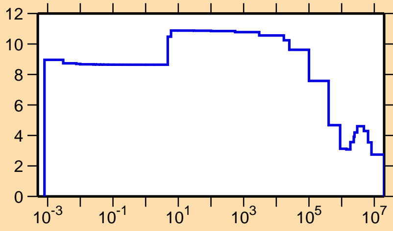
\sigma vs. E for ^{233}\text{Cm}(n,\text{el.})
