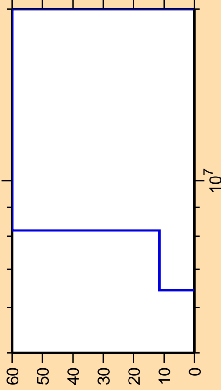
\Delta\sigma/\sigma vs. E for ^{234}\text{Cm}(n,d)
