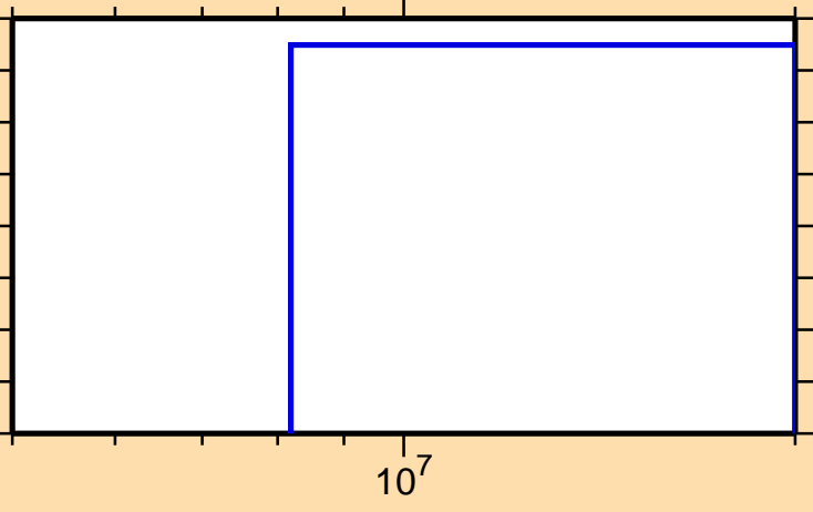
\sigma vs. E for ^{234}\text{Cm} (mt 45)
