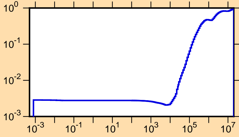
\mu vs. E for ^{235}\text{Cm}(\text{mt251})
