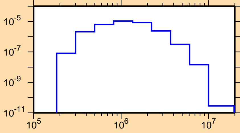
\sigma vs. E for ^{235}\text{Cm}(n,n_3)
