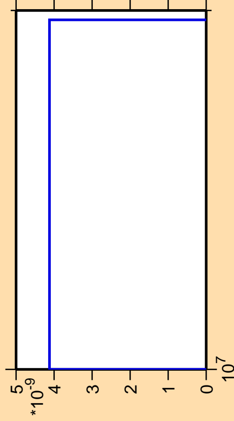
\Delta\sigma/\sigma vs. E for ^{235}\text{Cm} (mt 42)
