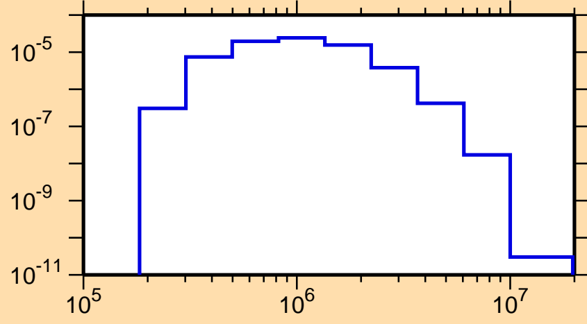
\sigma vs. E for ^{235}\text{Cm}(n,n_2)
