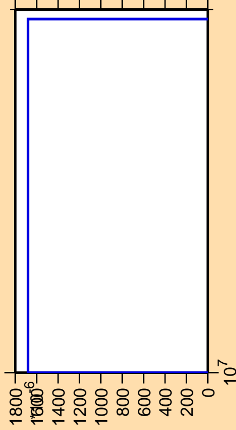
\Delta\sigma/\sigma vs. E for ^{235}\text{Cm}(\text{mt } 34)
