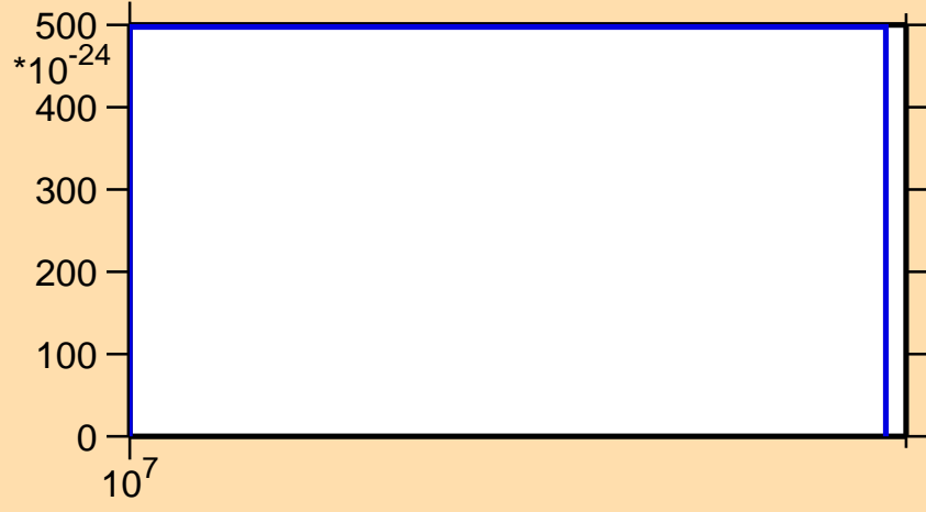
\sigma vs. E for ^{235}\text{Cm} (mt 42)
