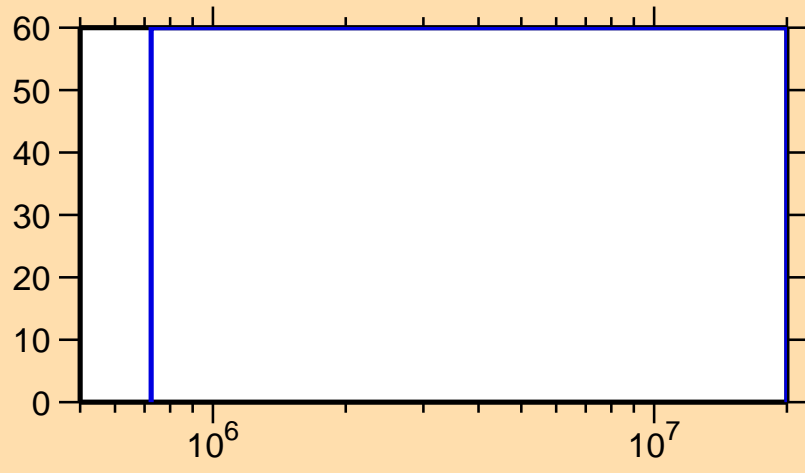
\Delta\sigma/\sigma vs. E for ^{236}\text{Cm}(n,ncont.)
