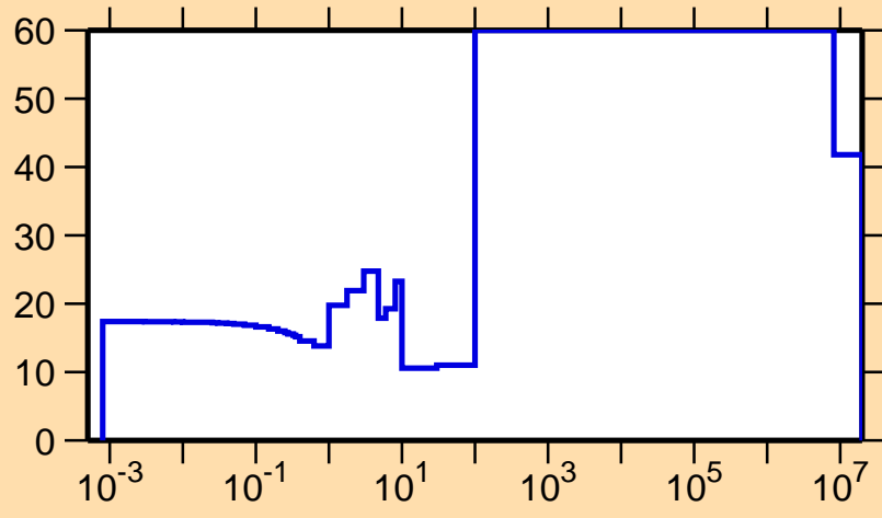
\Delta\sigma/\sigma vs. E for ^{236}\text{Cm}(n,\gamma)
