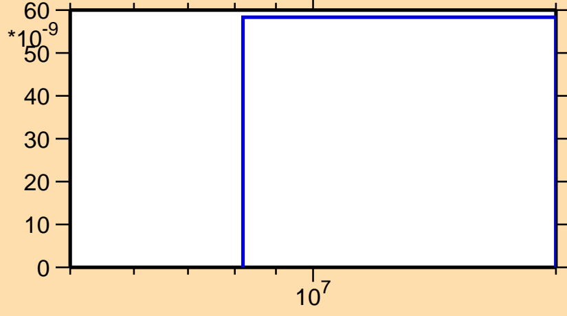
\sigma vs. E for ^{236}\text{Cm}(n,3n)
