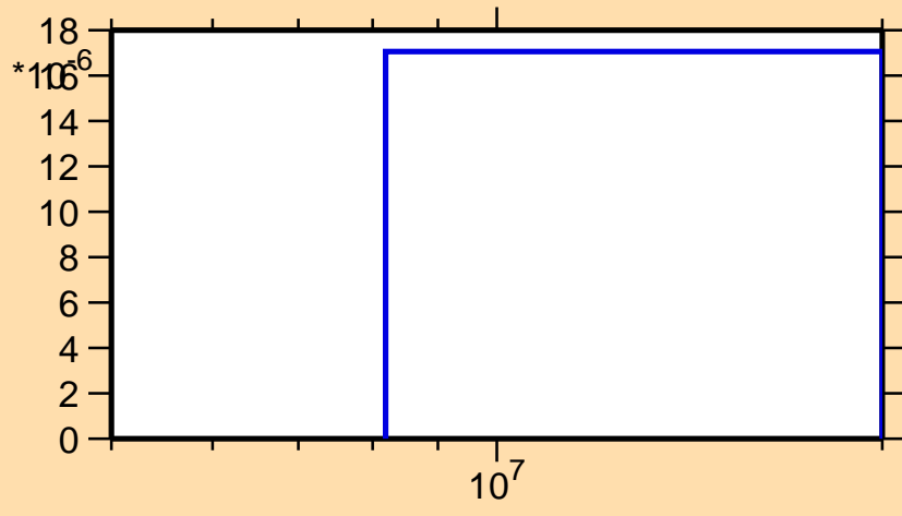
\sigma vs. E for ^{236}\text{Cm}(n,t)
