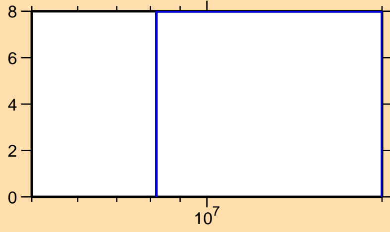
\Delta\sigma/\sigma vs. E for ^{236}\text{Cm}(n,\text{inel.})
