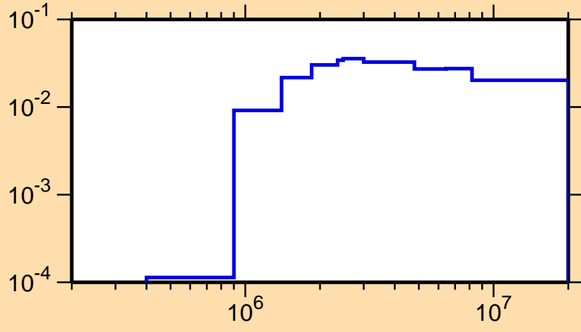
\sigma vs. E for ^{236}\text{Cm}(n,n\text{cont.})
