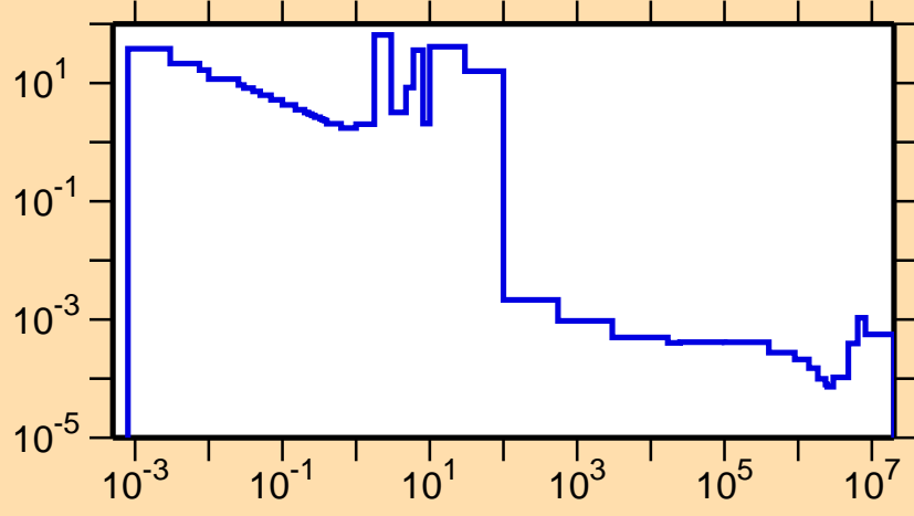
\sigma vs. E for ^{236}\text{Cm}(n,\gamma)
