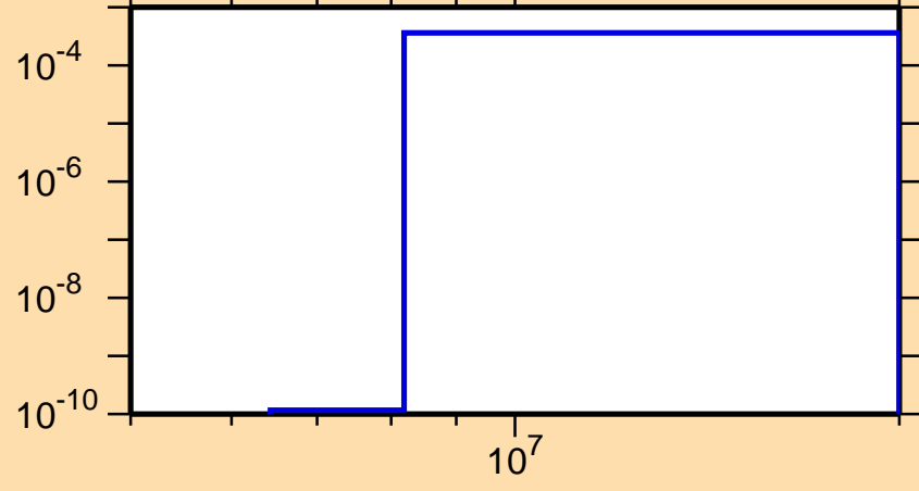
\sigma vs. E for ^{236}\text{Cm}(n,d)
