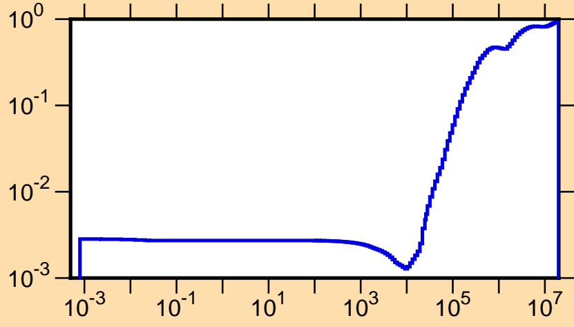
\mu vs. E for ^{237}\text{Cm}(\text{mt251})
