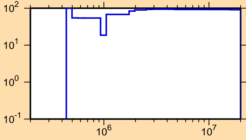
\Delta\sigma/\sigma vs. E for ^{237}\text{Cm}(n,ncont.)
