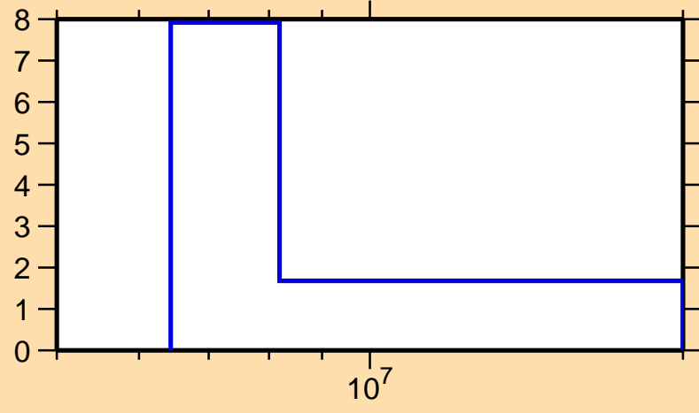
\Delta\sigma/\sigma vs. E for ^{237}\text{Cm}(n,\text{tot.})
