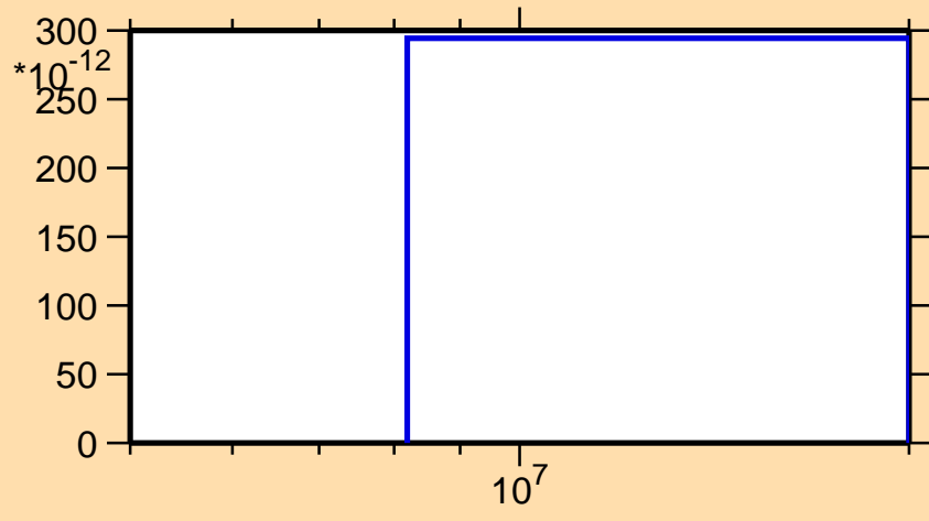
\sigma vs. E for ^{237}\text{Cm}(n,nd)
