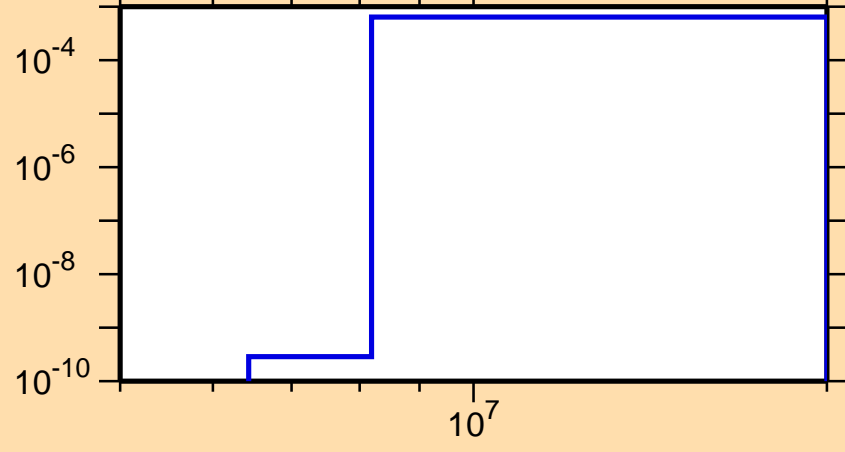
\sigma vs. E for ^{237}\text{Cm}(n,d)
