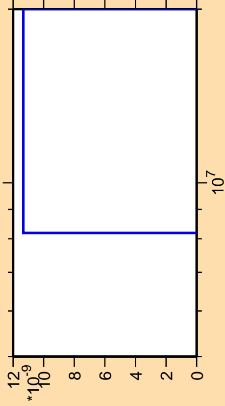
\Delta\sigma/\sigma vs. E for ^{237}\text{Cm} (mt 42)
