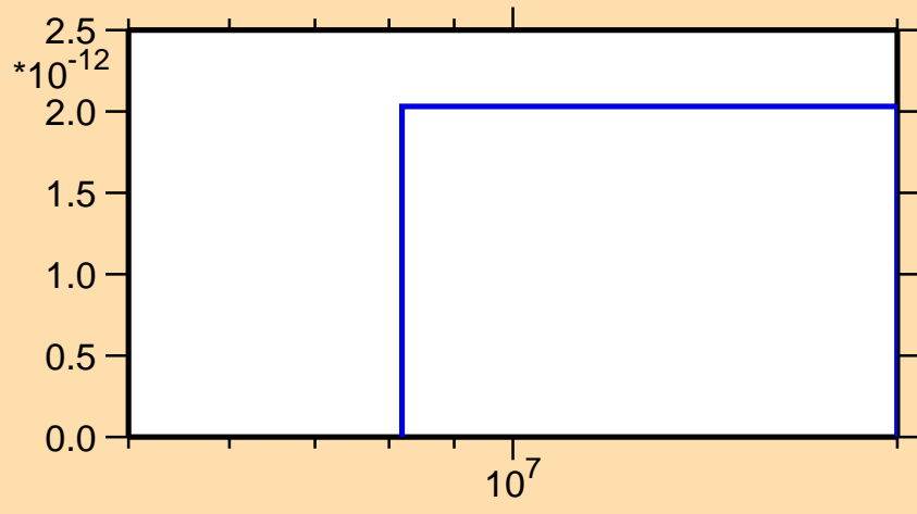
\sigma vs. E for ^{237}\text{Cm}(n,nt)
