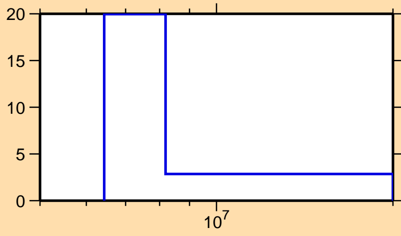
\Delta\sigma/\sigma vs. E for ^{237}\text{Cm}(n,el.)
