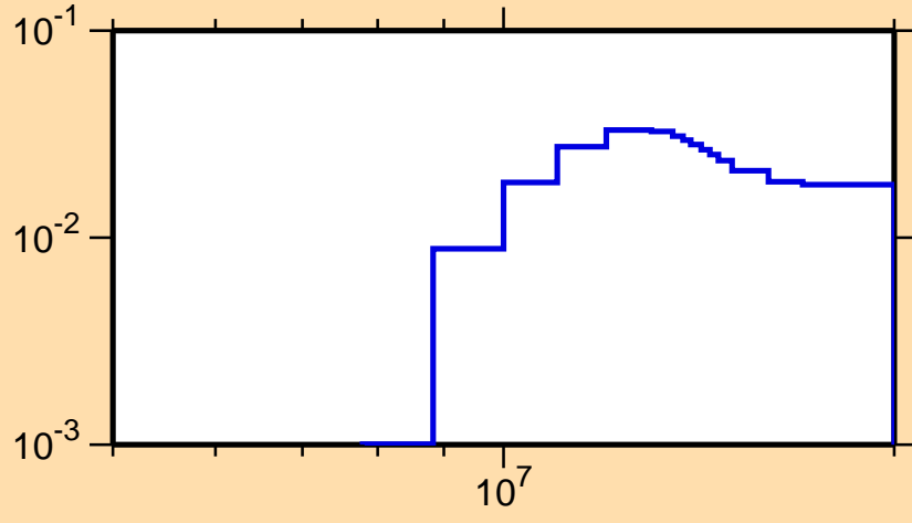
\sigma vs. E for ^{238}\text{Cm}(n,2n)
