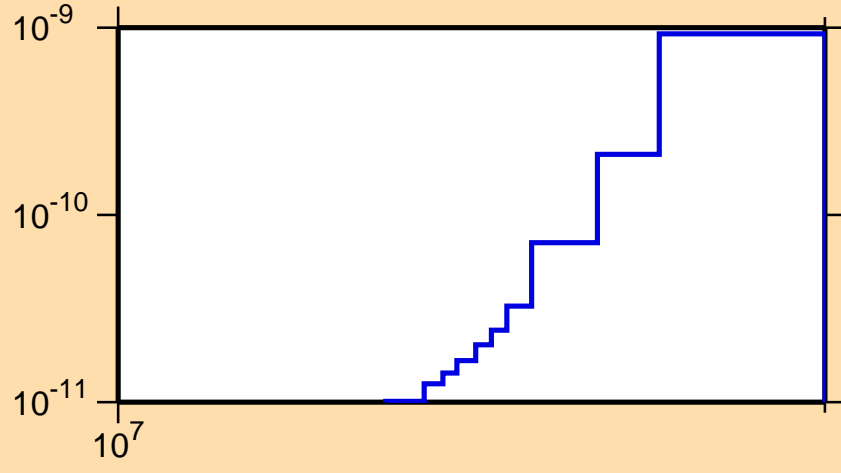
\sigma vs. E for ^{238}\text{Cm}(n,2n\alpha)
