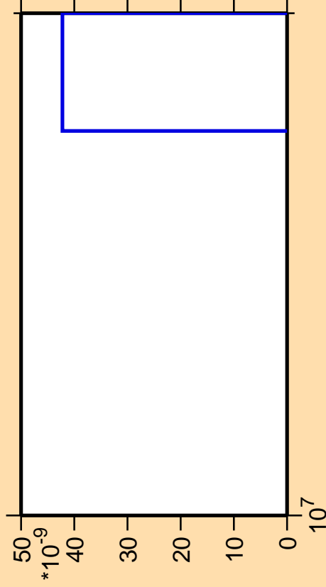
\Delta\sigma/\sigma vs. E for ^{238}\text{Cm} (mt 42)
