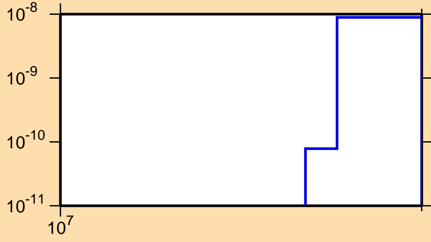
\sigma vs. E for ^{238}\text{Cm}(n,2np)
