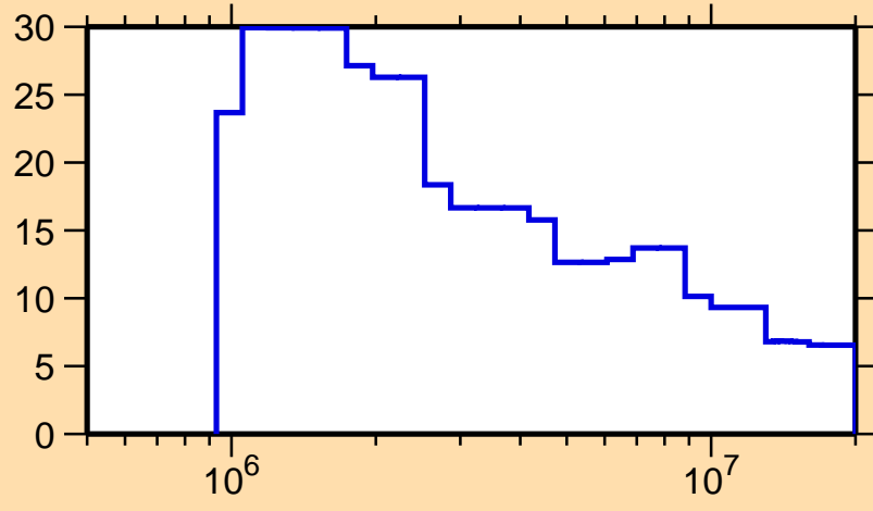
\Delta\sigma/\sigma vs. E for ^{238}\text{Cm}(n,\text{nonel.})
