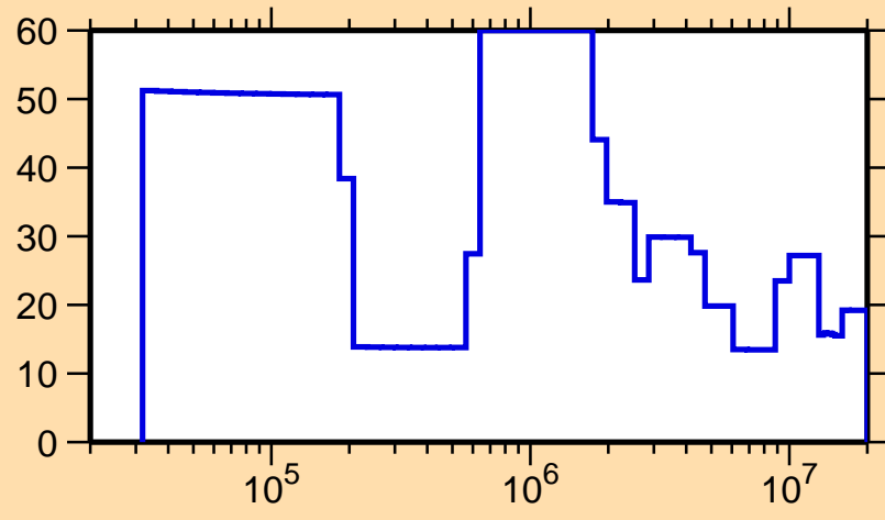
\Delta\sigma/\sigma vs. E for ^{238}\text{Cm}(n,\text{el.})
