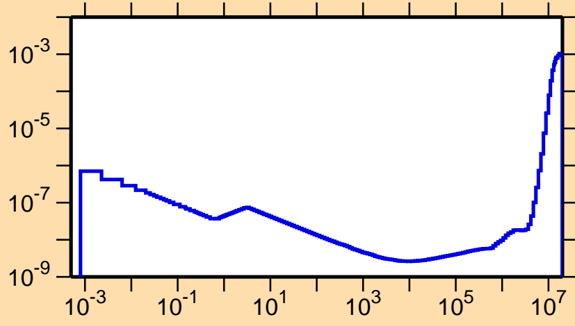
\sigma vs. E for ^{238}\text{Cm}(n,\alpha)
