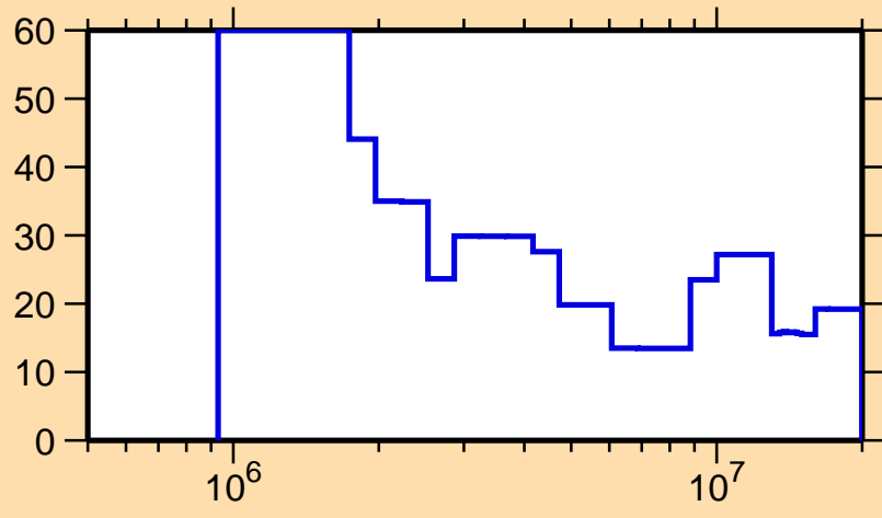
\Delta\sigma/\sigma vs. E for ^{238}\text{Cm}(n,el.)
