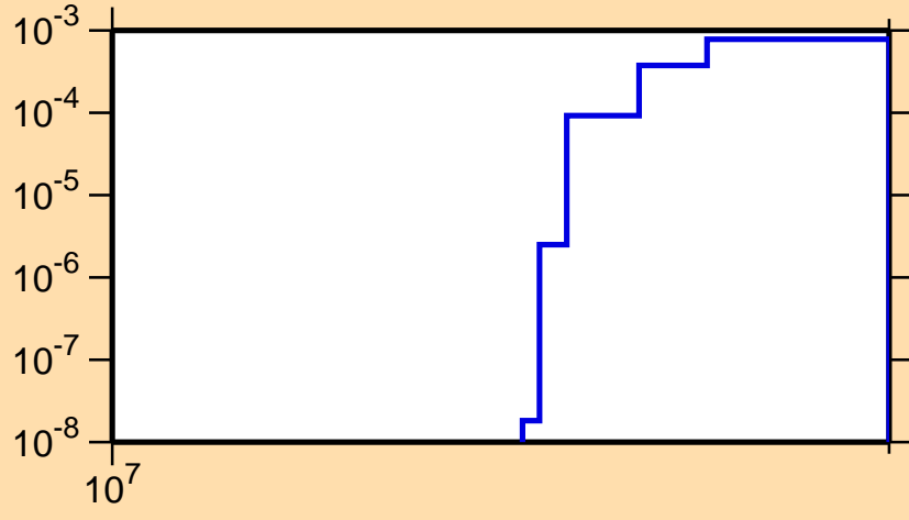
\sigma vs. E for ^{238}\text{Cm}(n,3n)
