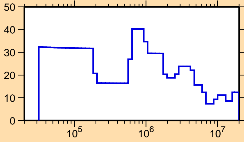
\Delta\sigma/\sigma vs. E for ^{238}\text{Cm}(n,\text{tot.})
