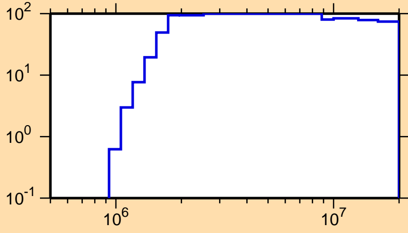
\Delta\sigma/\sigma vs. E for ^{238}\text{Cm}(n,p)
