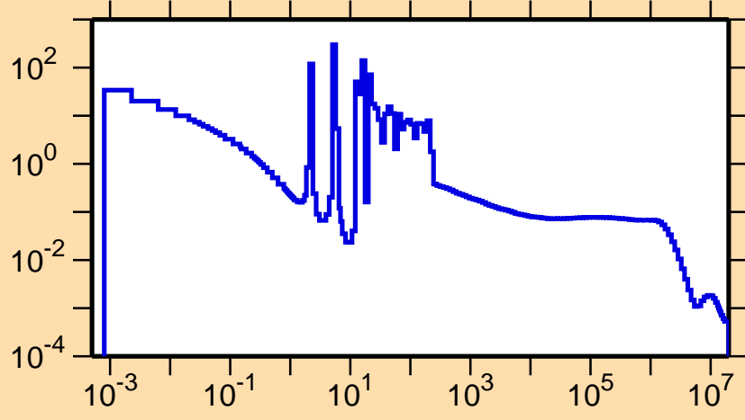
\sigma vs. E for ^{238}\text{Cm}(n,\gamma)
