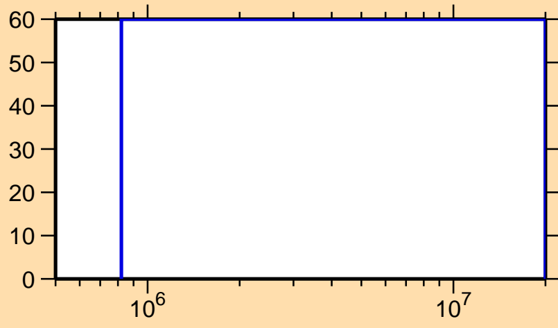
\Delta\sigma/\sigma vs. E for ^{238}\text{Cm}(n,n\text{cont.})
