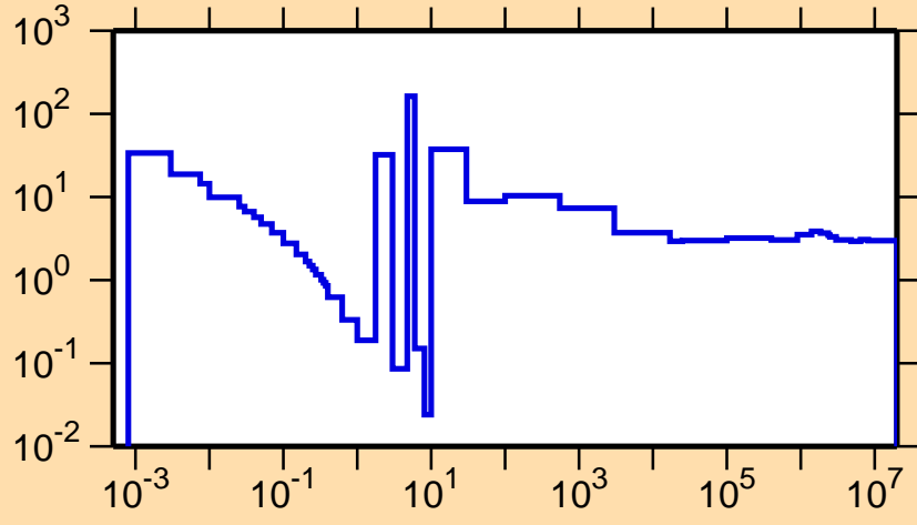
\sigma vs. E for ^{238}\text{Cm}(n,\text{nonel.})
