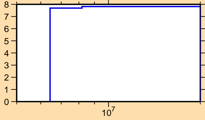
\Delta\sigma/\sigma vs. E for ^{238}\text{Cm}(n,\text{tot.})
