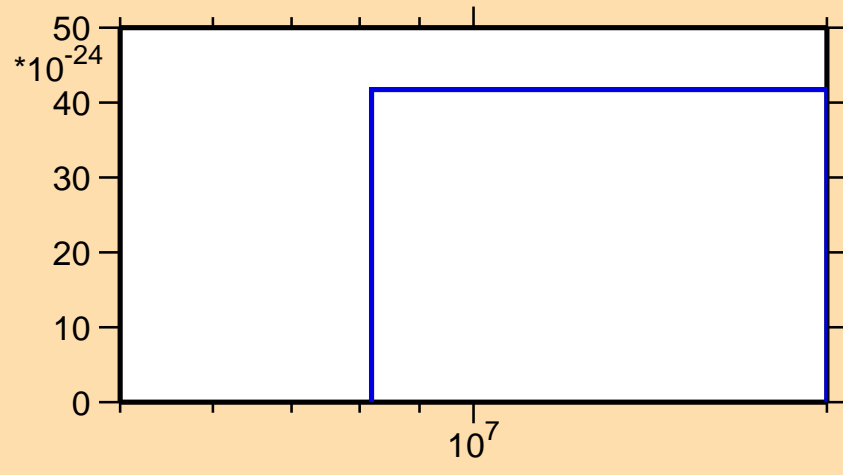
\sigma vs. E for ^{238}\text{Cm} (mt 42)
