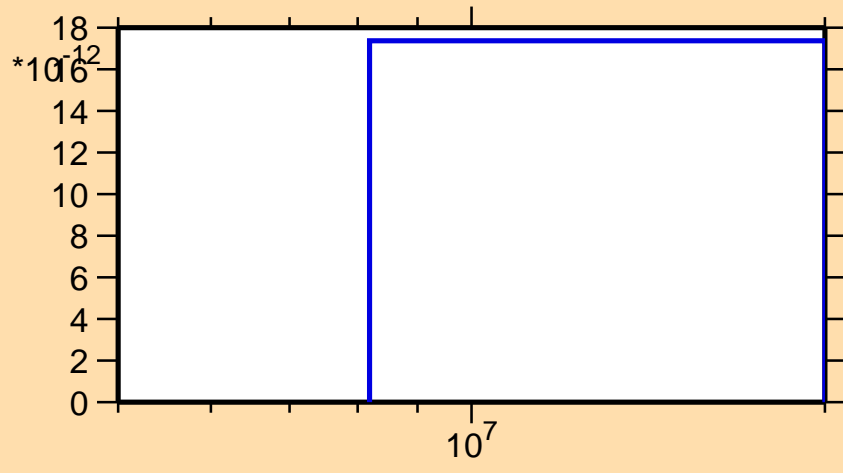
\sigma vs. E for ^{238}\text{Cm}(n,p\alpha)
