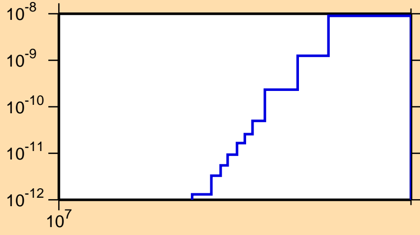
\sigma vs. E for ^{239}\text{Cm}(n,\text{He3})
