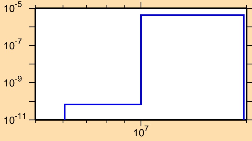
\sigma vs. E for ^{239}\text{Cm}(n,np)
