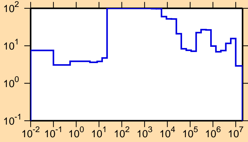
\Delta\sigma/\sigma vs. E for ^{239}\text{Cm}(n,tot.)
