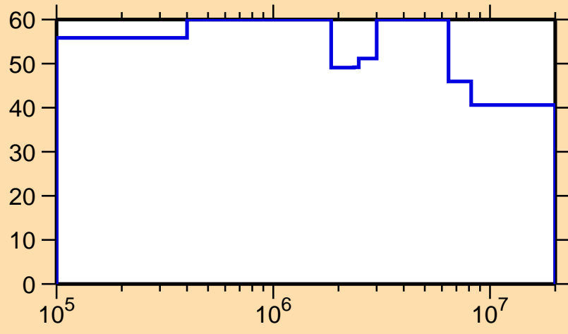
\Delta\sigma/\sigma vs. E for ^{239}\text{Cm}(n,n_1)
