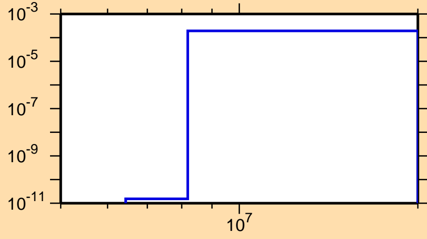
\sigma vs. E for ^{239}\text{Cm}(n,d)
