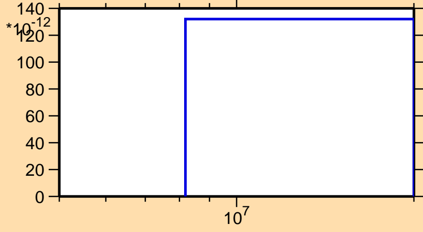
\sigma vs. E for ^{239}\text{Cm}(n,2n\alpha)
