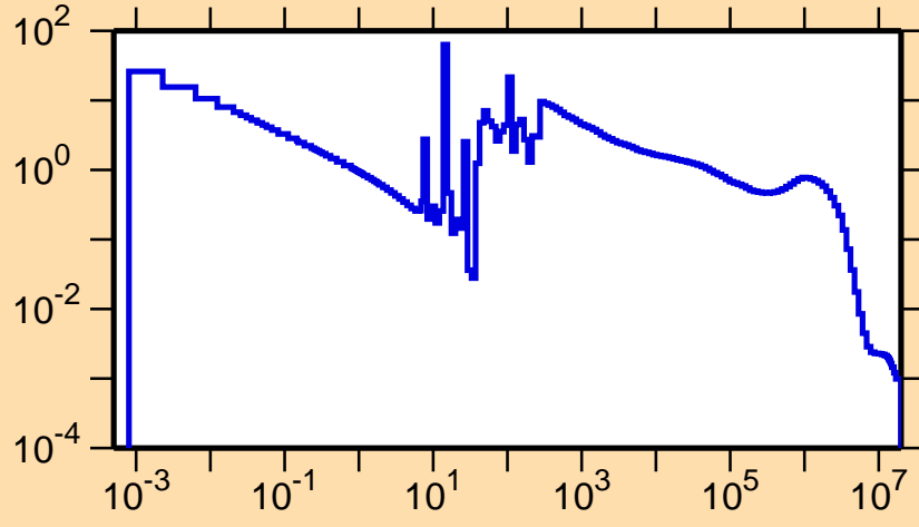
\sigma vs. E for ^{240}\text{Cm}(n,\gamma)
